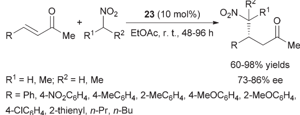
Scheme 29
