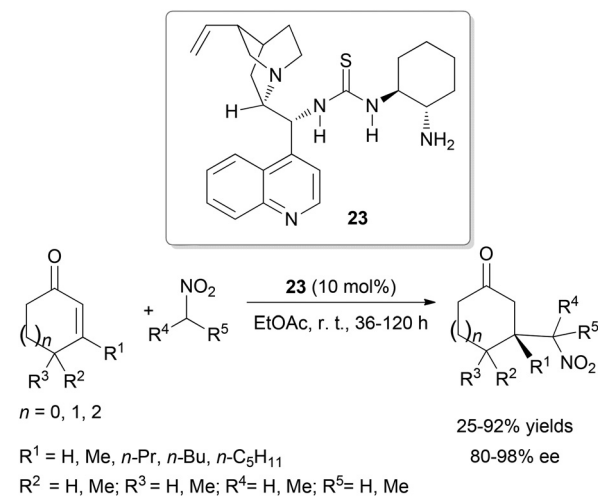
Scheme 28
