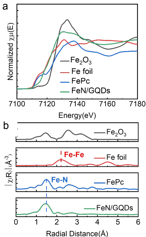
Figure 3. Atomic structural analysis of FeN/GQDs using a) X-ray absorption near edge structure (XANES) and b) extended X-ray absorption fine structure (EXAFS).
