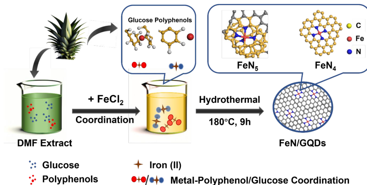
Scheme 1. Illustration of the synthesis process of FeN/GQDs nanozymes from ananas comosus leaves.
