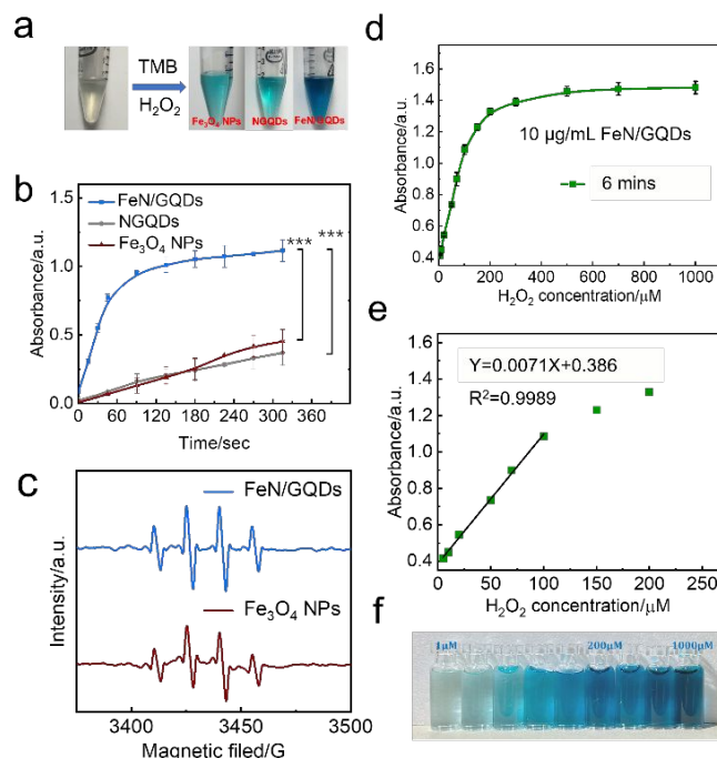
Figure 4. Peroxidase-like activity and kinetics analysis of FeN/GQDs. a) FeN/GQDs, NGQDs, and Fe 3 O 4 nanoparticles nanozymes exhibiting peroxidase-like activity through catalyzing the TMB substrate to produce colorimetric reactions. b) Reaction time-dependent absorbance curves of the TMB colorimetric reactions catalyzed by FeN/GQDs, NGQDs, and Fe 3 O 4 NPs respectively. Error bars represent standard deviation obtained from five independent experiments. ***: a p value < 0.01 means a 99.9% were considered statistically significant. c) EPR spectra showing OH• generation ability of FeN/GQDs with DMPO as the trapping agent, in comparison with Fe 3 O 4 nanoparticles (NPs). d) to f) TMB assay for H 2 O 2 detection, where each sample contains 10 mg/mL FeN/GQDs, 0.3 mM TMB, and 1 mM pH3.6 PBS buffer. d) UV-vis absorbance change of FeN/GQDs as a function of H 2 O 2 concentration. e) The linear region of the absorbance curve shown in a): over the 99% confidence interval, showing the absorbance change with the increase in H 2 O 2 concentration from 5 μM to 100 μM. f) A photograph of FeN/GQDs samples with varying H 2 O 2 concentrations, showcasing the color change of the H 2 O 2 /TMB/FeN-GQDs reaction system as the concentration of H 2 O 2 increases. The color change is a visual representation of the catalytic activity of FeN/GQDs in the presence of varying amounts of H 2 O 2 .
