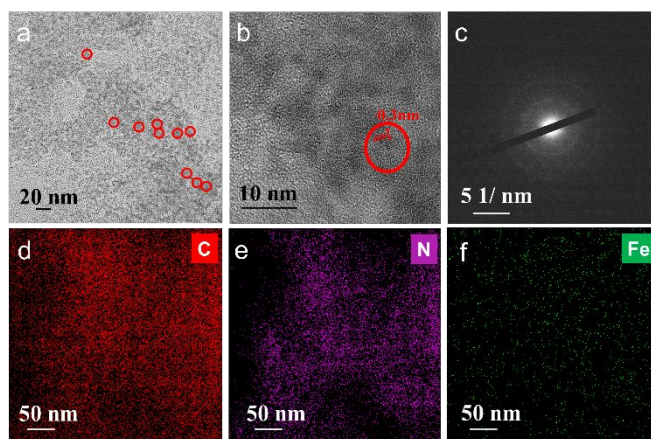
Figure 1. The morphology and elementary distribution of FeN/GQDs. a) TEM image of FeN/GQDs. b) High-resolution TEM image of FeN/GQDs. c) SEAD patterns of FeN/GQDs. d-f) Corresponding EDS element mapping of FeN/GQDs: carbon (d), nitrogen (e), and Iron (f).
