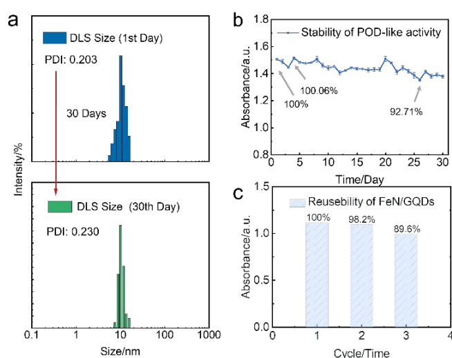
Figure 6. Stability and reusability of FeN/GQDs nanozymes. a) Colloidal stability of FeN/GQDs assessed by measuring the hydrodynamic size distribution of FeN/GQDs using dynamic light scattering. Top panel: the size distribution at day 0; bottom panel: size distribution at day 30. The size distribution exhibited no significant change after 30 days of storage at room temperature. b) The stability of FeN/GQDs catalytic activity assessed by measuring the absorbance at 652nm over a period of 30 days. FeN/GQDs are stored at room temperature. c) The reusability assessment of FeN/GQDs by measuring the absorbance of FeN/GQDs after multiple rounds of washing. Considering the first-time absorbance as 100% activity, the second time and third time cycle activities have the 98.2% and 89.6% activities.
