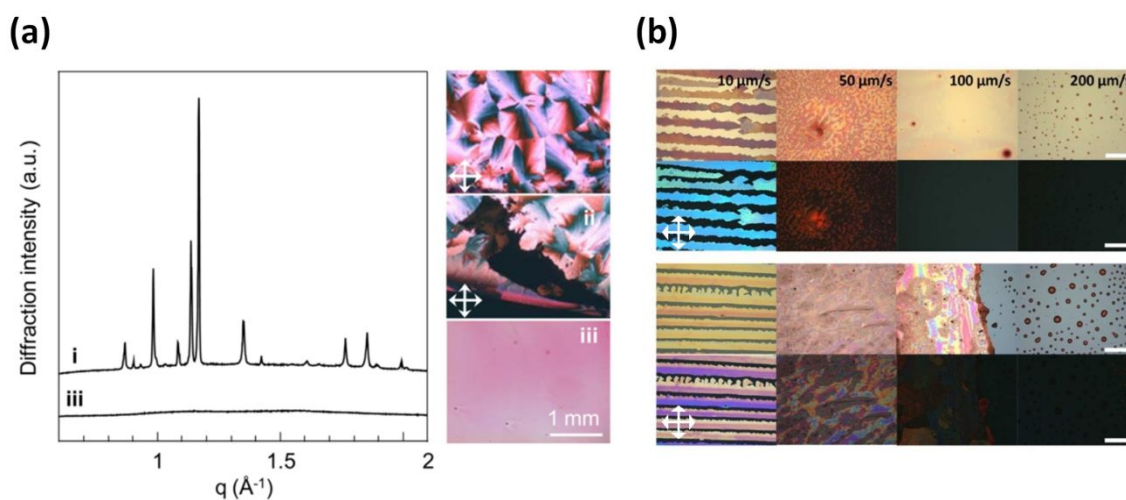
Fig. 3. (a) TES ADT thin films drop cast at 5 °C (i), room temperature (ii) and 40 °C (iii). X-ray diffraction patterns (left panel) and polarized optical micrographs (right panel) for scenario (i) and (iii) (reproduced from Ref. 7). (b) Polarized optical micrographs of TES ADT thin films obtained on \text{Al}_2\text{O}_3 (top panel) and \text{SiO}_2 substrates (bottom panel) via dip-coating using various dipping speeds from a dichloromethane solution (reproduced from Ref. 17).
