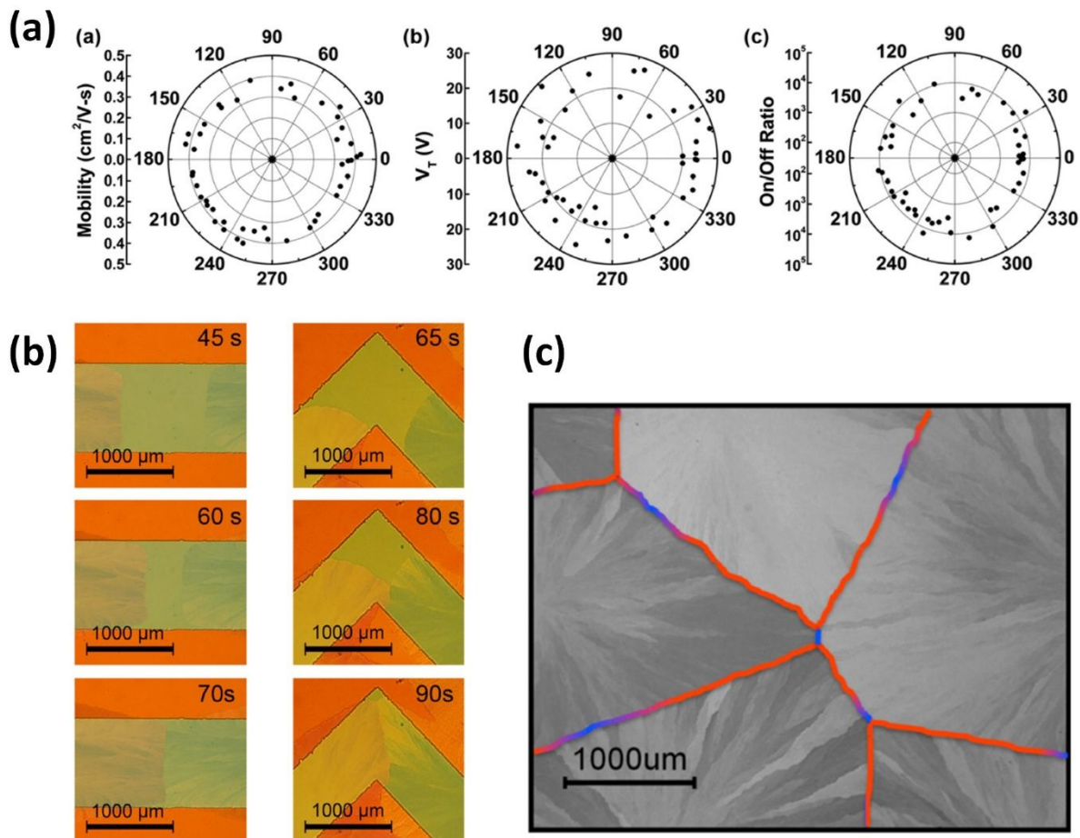
Fig. 7. (a) Pole figures showing the low directional dependence of transistor mobility, threshold voltage and ON-OFF ratio measured within one single TES ADT spherulite (reproduced from Ref. 30). (b) Optical micrographs of TES ADT thin films deposited on surface-energy patterned substrates illustrating formation of high-angle and low-angle interspherulite boundaries. (c) Optical micrograph of a TES ADT thin film where high-angle (blue) and low-angle interspherulite boundaries (red) are readily identified (reproduced from Ref. 36).
