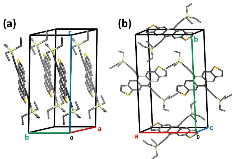
Fig 6. Crystalline packing in \alpha - (a) and \beta - TES ADT (b).
