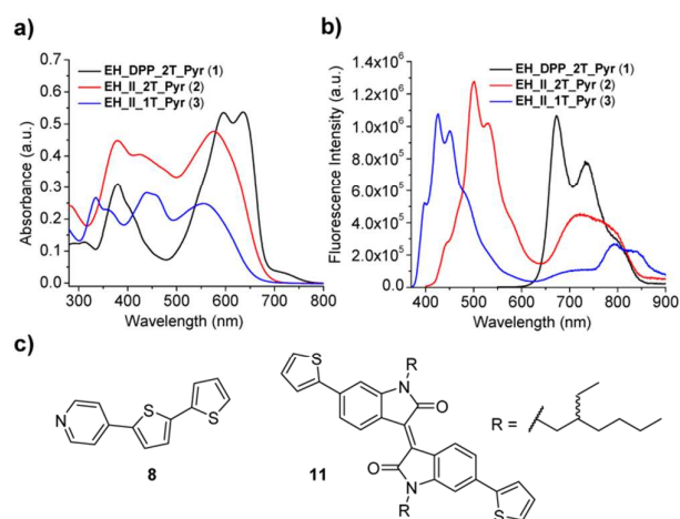
Fig. 4 Absorption (a) and fluorescence (b) spectra of 1 , 2 , and 3 in THF (10 \mu M) (molar extinction coefficient ( \epsilon ) of 1 = 4.8 \times 10^4 \text{ M}^{-1}\cdot\text{cm}^{-1} , 2 = 3.9 \times 10^4 \text{ M}^{-1}\cdot\text{cm}^{-1} , and 3 = 2.6 \times 10^4 \text{ M}^{-1}\cdot\text{cm}^{-1} ), (c) chemical structure of end group 8 and core unit 11 used as test compounds. \lambda_{\text{excitation}} of 1 = 390 nm, 2 = 380 nm, and 3 = 355 nm.
