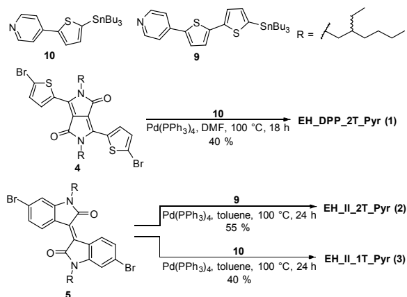
Scheme 1 Synthesis of EH_DPP_2T_Pyr ( 1 ), EH_II_2T_Pyr ( 2 ), and EH_II_1T_Pyr ( 3 ). Additional synthetic details and intermediates can be found in the Supplementary Information (e.g., Fig. S1).
