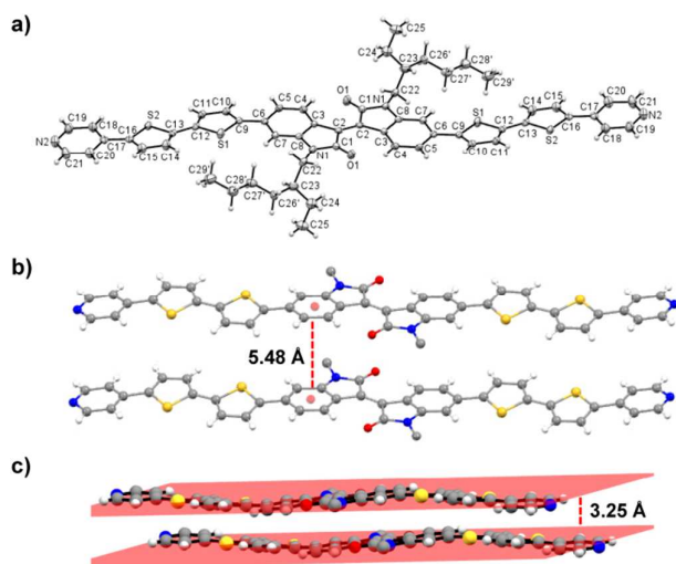
Fig. 2 X-ray crystal structure of compound 2 . (a) The full molecule is shown using thermal displacement ellipsoids at 40%. (b) packing diagram showing the distance between adjacent ring centroids, and (c) packing diagram showing the distance between molecular planes (side chain disorder has been removed for clarity in a), and alkyl chains are omitted in b), c) for clarity).
