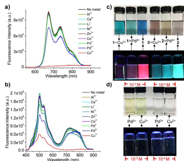
Fig. 7 Fluorescence spectra showing the extent of luminescence quenching of 1 (a) and 2 (b) with 2 equiv of metal ions. ( \lambda_{\text{excitation}} of compound 1 = 390 nm; compound 2 = 380 nm). Photographs which show, (c) color changes of solutions of 1 and 2 upon addition of 10 equiv ( 10^{-4} M) of \text{Pd}^{2+} and \text{Cu}^{2+} ; (d) the color of neat \text{Pd}^{2+} and \text{Cu}^{2+} solutions at different concentrations ( 10^{-3} M and 10^{-4} M) (for c and d, top pictures : under ambient white light, bottom pictures : with UV lamp ( \lambda = 365 nm) excitation). Metal complexes used: \text{AlCl}_3 , \text{LiCl} , \text{CaCl}_2 , \text{ZnCl}_2 , \text{Co}(\text{OAc})_2 \cdot 4\text{H}_2\text{O} , \text{Ni}(\text{OAc})_2 \cdot 4\text{H}_2\text{O} , \text{Pd}(\text{dba})_2 , \text{Pd}(\text{OAc})_2 , \text{CuCl}_2 .
