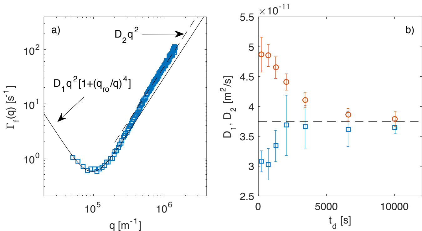
Fig. 8 a) Correlation rate of the fast relaxation mode of concentration fluctuations in a diffusing non-equilibrium colloidal suspension as a function of the scattering wave-vector q , measured at t_d = 690 s after the beginning of diffusion. The continuous line is the best fit of the low- q data with Eq. 10, which provides an estimate for the roll-off wave-vector q_{ro} and for the diffusion coefficient D_1 . The dashed line is a fit of the high- q data with \Gamma(q) = D_2 q^2 , where D_2 > D_1 . b) Diffusion coefficients D_1 (squares) and D_2 (circles) extracted as shown in panel a) at different times during diffusion. The corresponding values for q_{ro} are reported in Fig. 5b as orange circles.
