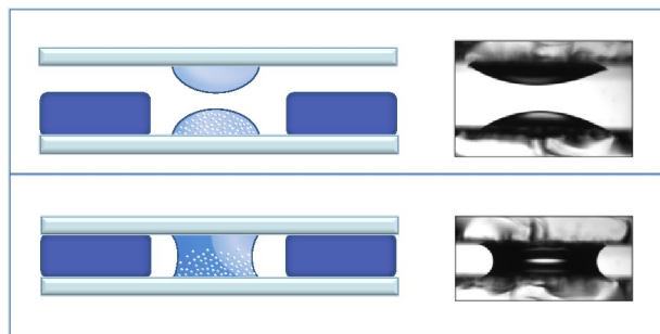
Fig. 3 Schematic representation (left) and photographs (right) of the measurement cell before (a) and after (b) the final assembly. a) a 17 \mu\text{l} drop of the colloidal suspension is deposited at a center of glass slide while an identical drop of distilled water is deposited at the center of another slide. On the bottom slide a gasket, obtained by a thin soft rubber sheet with a circular hole, is positioned. b) The two drops are then aligned and put in contact. Immediately, a liquid bridge forms between the two slides and the diffusion process starts.
