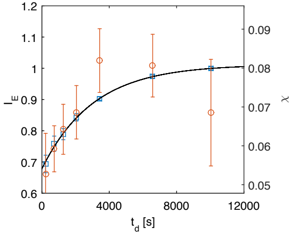
Fig. 6 Right axis: Osmotic compressibility \chi (red circles) obtained during diffusion obtained from inversion of Eq.12. Left axis: equilibrium scattering intensity (blue squares) obtained from the large- q behavior in Fig. 5a.
