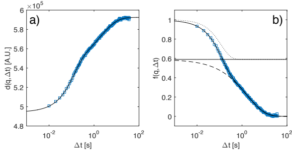
Fig. 4 a) Experimental results (blue squares) for the image structure function (a) and intermediate scattering function (b) measured at q = 0.45 \mu\text{m}^{-1} , and at time t_d = 2010 \text{ s} from the beginning of the diffusion process. The continuous line is the best fitting curve of the experimental data to a double exponential process as given by Eqs. 17 and 18. In (b) we decompose the decay described by Eq. 18 in its two components, a fast one (dotted line) and a slow one (dashed line), with the horizontal line representing the amplitude a_s
