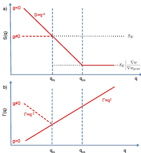
Fig. 1 Schematic diagram showing the scaling regimes for the static structure factor S(q) (a) and the decay rate \Gamma(q) (b) of the concentration fluctuations in the hydrodynamic range qR \ll 1 for a colloidal suspension of particles with radius R subjected to a macroscopic concentration gradient \nabla w . Both plots are in bi-logarithmic scale. The continuous line represents schematically the situation in the absence of buoyancy effects ( g = 0 ). The dashed line depicts the effect of buoyancy, which appears only for q < q_{ro} . Here we depict only the most typical case q_{ro} < q_{co} . A similar diagram can be drawn for q_{ro} > q_{co} , as shown in Fig. 2 only for the case g \neq 0 .
