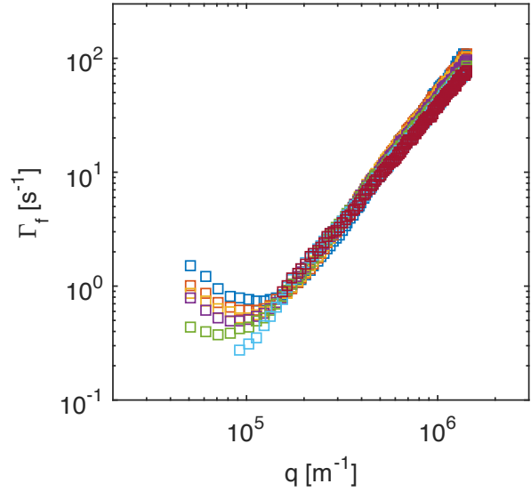
Fig. 7 Correlation rate of the fast relaxation mode of concentration fluctuations in a diffusing non-equilibrium colloidal suspension as a function of the scattering wave-vector q , for different times t_d = 180, 690, 1230, 2010, 3390, 6540, 10000 s after the beginning of diffusion.
