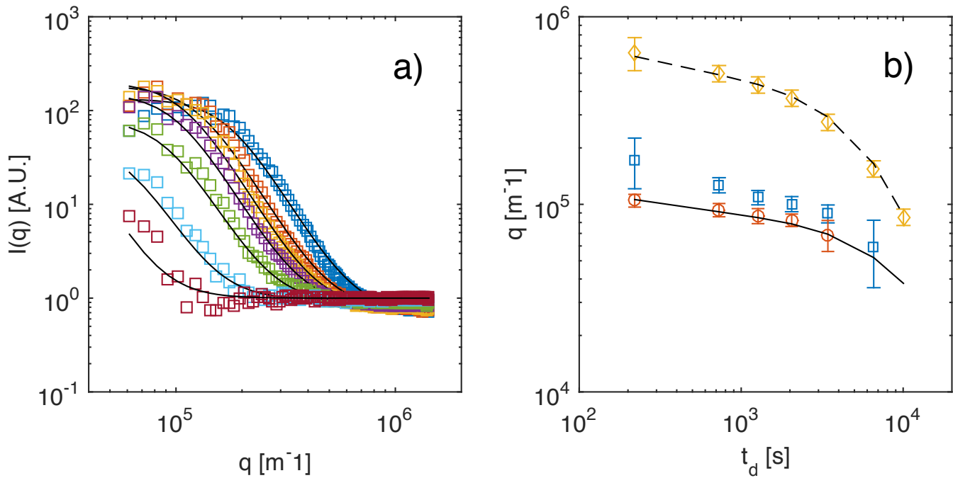
Fig. 5 (a) Scattering intensity I_f(q) obtained for a diffusing colloidal suspension at various times t_d from the beginning of diffusion: t_d = 180, 690, 1230, 2010, 3390, 6540, 10000 s (from top to bottom). Continuous lines are best fits to Eq. 9. Data for I_s(q) are shown in ESI. (b) Roll-off wave-vector q_{ro} as function of the time t_d elapsed from the beginning of diffusion, as obtained from the static (blue squares) and from the dynamic (orange circles) analysis of the NEF. The continuous line is a theoretical prediction from Eq. 11, evaluated for z corresponding to the sample mid-plane. Yellow diamonds represent the crossover wave-vector q_{co} . The dashed line is the theoretical prediction from Eq. 12, again calculated for z corresponding to the sample mid-plane. In addition, the osmotic compressibility \bar{\chi} is assumed to remain constant during diffusion.
