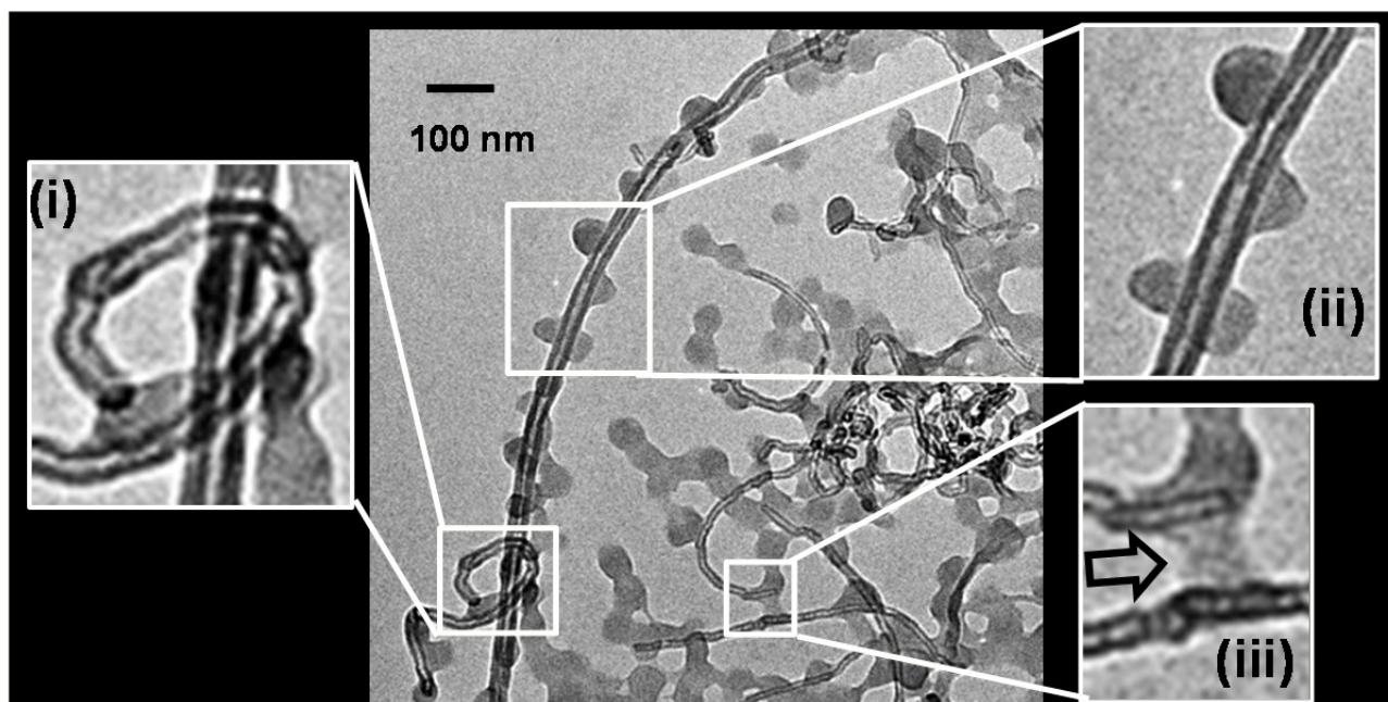
Fig. 3. Evidence for an attractive MG-CNT interaction from TEM. The TEM images are of dried SX MG1/CNT 1.0 after dilution. The pH of the mixed MG1/CNT dispersion before dilution was 6.8. The insets show (i) entangled CNTs with one CNT threading another looped CNT, (ii) MGs adsorbed on a CNT and (iii) a MG particle bridging two CNTs.
