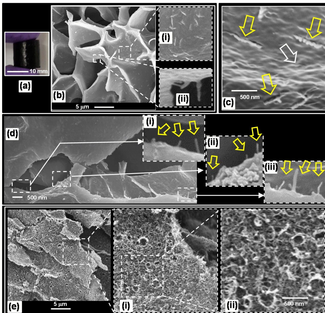
Fig. 4. DX MG1/CNT morphology. (a) DX MG1/CNT 1.0 cylinder. (b) and (c) show SEM images of freeze-dried DX MG1/CNT 0.5 . The insets for (b) show rod-like features ((i) and (ii)). (c) shows a higher magnification image from (b). The white and yellow arrows show, respectively, MG particles and deformation patterns caused by CNTs (see text). (d) A sample was fractured and then freeze-dried and the image shows a fracture surface. The insets ((i) to (iii)) show CNTs protruding from the fracture surface (identified with arrows). (e) shows SEM images for DX MG1/CNT 0.5 gel after heating at 850 °C in N 2 . The insets ((i) and (ii)) show increasing magnifications of the entangled CNT mesh.
