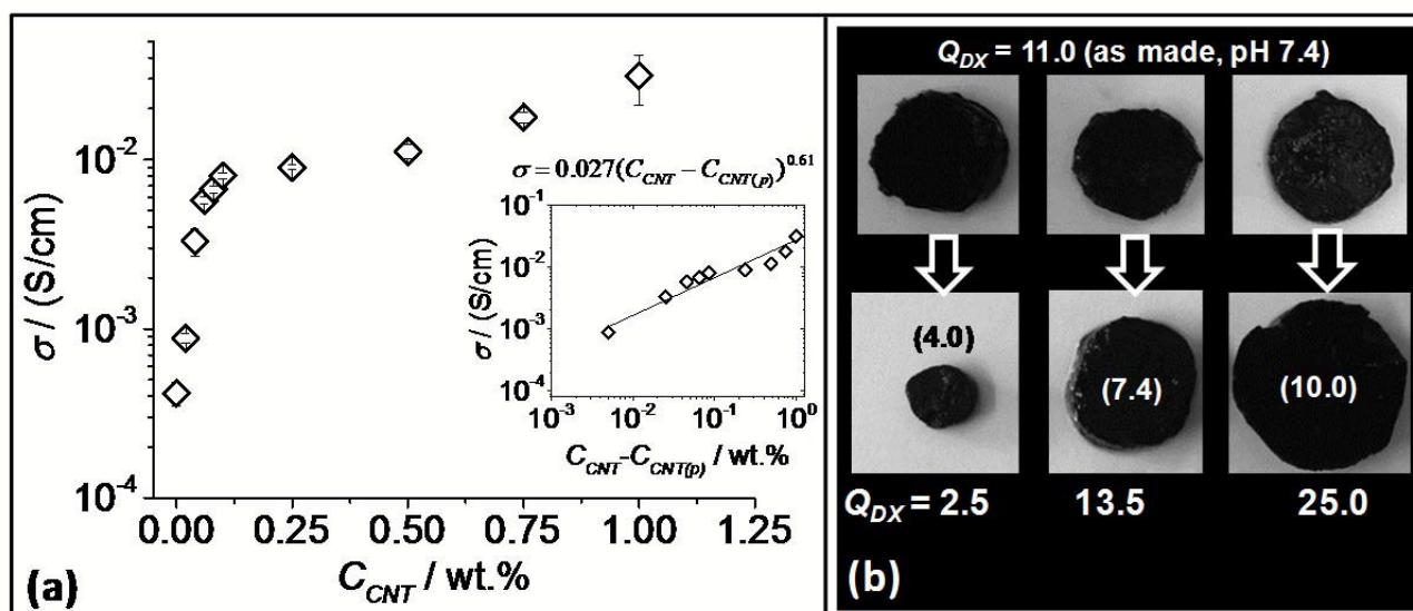
Fig. 5. Conductive gel composite properties. (a) Conductivity variation with CNT concentration for DX MG1/CNT y . The inset shows a fit for the data to the percolation model (equation (1)). At least three samples were tested for each data point and the error bars include the minimum and maximum values. (b) pH-responsive swelling of DX MG1/CNT 1.0 after three samples prepared at pH 7.4 (top row) were placed in buffer solution. The pH values for the latter are shown in brackets for the bottom row. Q_{DX} is the equilibrium gel composite volume swelling ratio.
