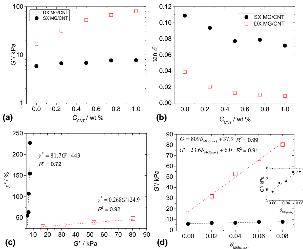
Fig. 6. Rheological properties for SX MG1/CNT and DX MG1/CNT. Variation of G' (a) and (b) \tan \delta with CNT concentration. These values were measured at a frequency of 1 Hz. (c) shows the critical strain as a function of G' . (d) Variation of G' with maximum average fractional coverage of the MG particles with CNT (See text). The legends for (a) and (b) also apply to (c) and (d). The inset for (d) shows an expanded view of the SX MG1/CNT data.
