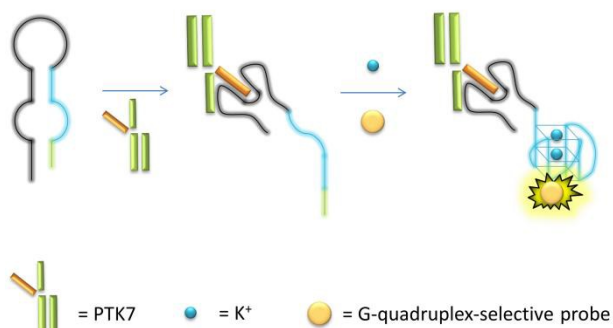
Scheme 1 Schematic representation of the G-quadruplex-based luminescence sensing platform for PTK7 detection.
