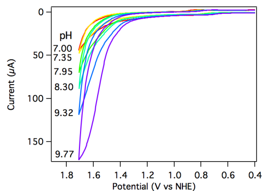
Figure 5. CV of 0.25 mM [Ru(Py 3 PO)(bpy)(OH 2 )] 2+ at pH 7.00 (red), 7.35 (yellow), 7.95 (green), 8.30 (teal), 9.32 (blue), and 9.77 (purple) at 100 mV·s -1 . Conditions: 0.1 M phosphate, 3 mm glassy carbon working electrode, Pt wire counter electrode, Ag/AgCl reference electrode.
