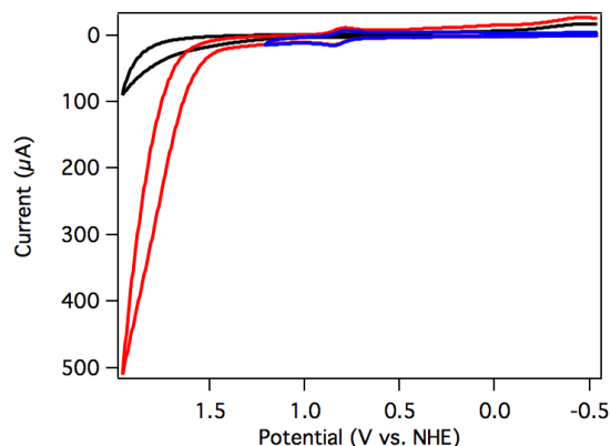
Figure 3. CV of [\text{Ru}(\text{Py}_3\text{PO})(\text{bpy})(\text{OH}_2)]^{2+} ( 3 ) swept anodically to 1.95 V (red) and 1.2 V (blue) vs. NHE. A catalyst-free background scan is shown in black. The reduction near -0.5 V is assigned to \text{O}_2 reduction. Conditions: 250 \text{ mV} \cdot \text{s}^{-1} scan rate, pH 7 0.1 M phosphate buffer, 3 mm
