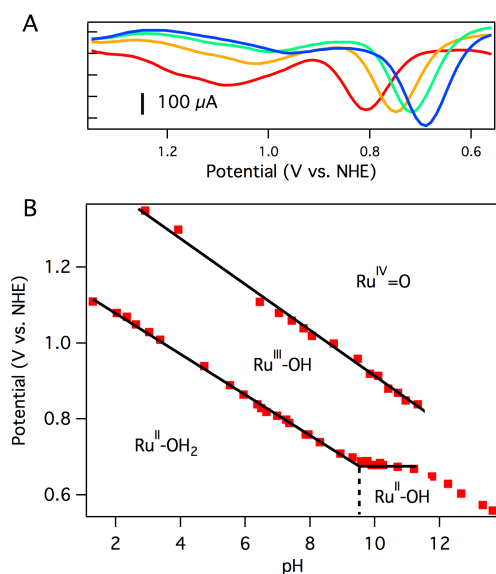
Figure 2. Differential pulse voltammograms at pH 7.0 (red), pH 8.0 (orange), pH 8.7 (green), and pH 9.5 (blue) (A) and resulting Pourbaix diagram (B) of [\text{Ru}(\text{Py}_3\text{PO})(\text{bpy})(\text{OH}_2)]^{2+} ( 3 ). Solid black lines are linear fits to portions of the data. The slope of the first oxidation (pH 1-9) is 54 mV per pH unit. The slope of the second oxidation (pH 2-10) is 60 mV per pH unit. The dashed vertical line represents the \text{p}K_a of aquo 3 . Conditions: 0.1 M phosphate, 3 mm glassy carbon disc working electrode, Pt wire counter electrode, Ag/AgCl reference electrode.
