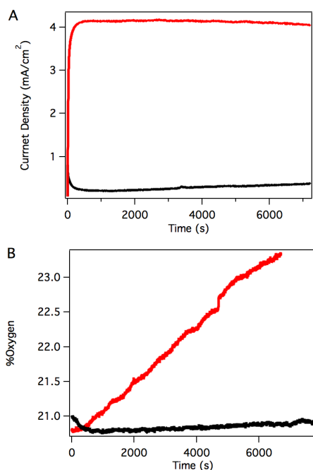
Figure 4. A: Controlled potential electrolysis (CPE) of solutions containing 3 (red) and without catalyst (black) at 1.8 V vs. NHE. B: Headspace O 2 fluorescence detection during CPE of solutions containing 3 (red) and without catalyst (black). Conditions: 0.45 mM catalyst, 0.1 M phosphate at pH 7, 1.4 cm 2 planar ITO electrode.
