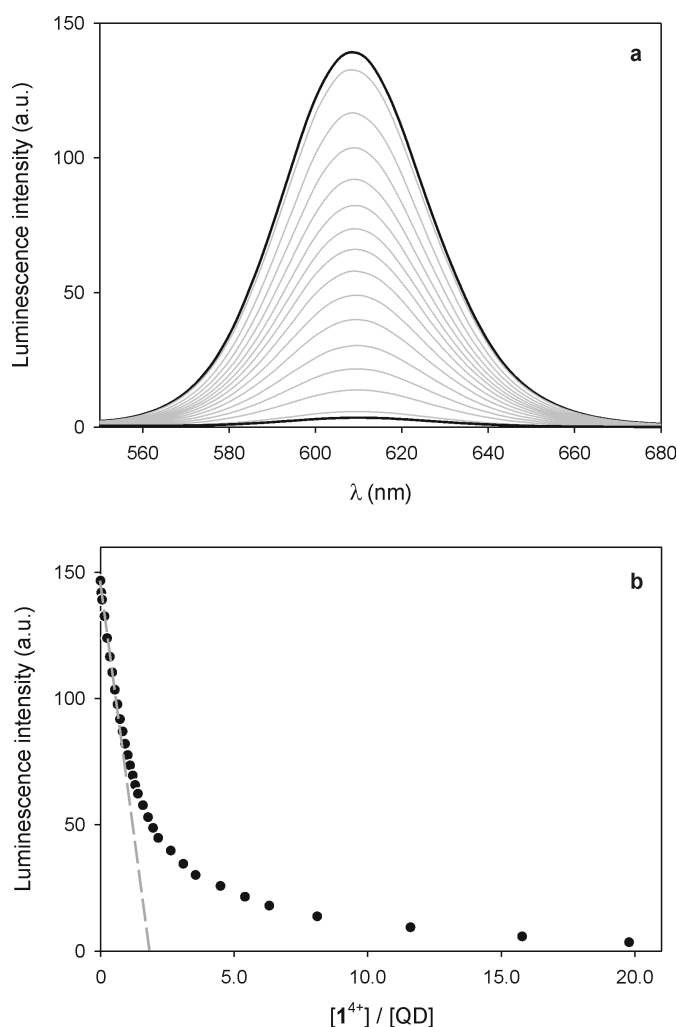
Fig. 3 (a) Luminescence spectral changes observed upon titration of 0.47 \mu\text{M} CdSe-ZnS QDs with \mathbf{1}^{4+} . (b) Titration plot obtained from the QD luminescence intensity at 608 nm in the presence of increasing amounts of \mathbf{1}^{4+} . The dashed line shows the tangent to the first part of the curve (it is a guide for the eye, not a fit). Conditions: air equilibrated \text{CHCl}_3/\text{CH}_3\text{CN} 9:1, room temperature, \lambda_{\text{exc}} = 500 nm.
