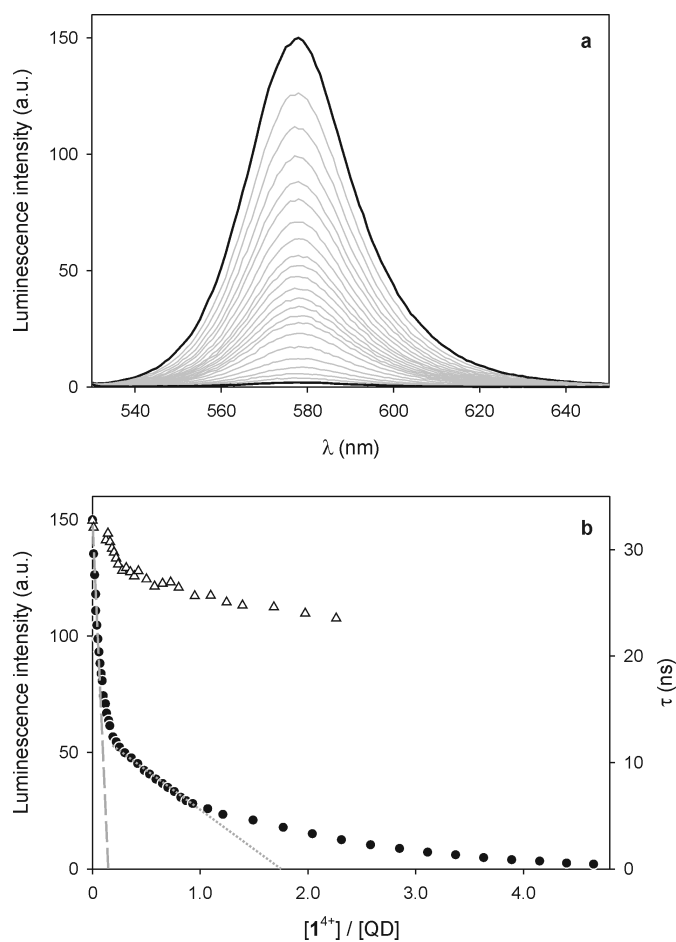
Fig. 1 (a) Luminescence spectral changes observed upon titration of 1.5 \mu\text{M} CdSe QDs with \mathbf{1}^{4+} . (b) Filled circles, left scale: titration plot obtained from the QD luminescence intensity at 578 nm in the presence of increasing amounts of \mathbf{1}^{4+} . The dashed and dotted lines show the tangent to the curve at two different slopes and are a guide for the eye, not a fit. Empty triangles, right scale: titration plot obtained from the luminescence lifetime values corresponding to the CdSe emission. Conditions: air equilibrated \text{CHCl}_3/\text{CH}_3\text{CN} 9:1, room temperature, \lambda_{\text{exc}} = 500 nm.
