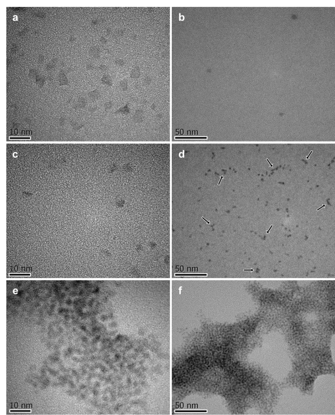
Fig. 5 TEM Images recorded on substrates obtained from deposition of dilute solutions of (a, b) CdSe QDs, (c, d) CdSe QDs and 1^{4+} in a 1:1 ratio, and (e, f) CdSe QDs and 1^{4+} in a 1:4 ratio. Arrows in (d) indicate small QD aggregates. Scale bar is 10 nm for (a, c, e) and 50 nm for (b, d, f).
