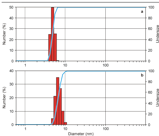
Fig. 4 Differential (red bars) and cumulative (blue line) number distributions of particle size obtained from DLS measurements for the CdSe QDs (a) alone and (b) in the presence of 0.5 equivalents of 1^{4+} . Conditions: air equilibrated \text{CHCl}_3/\text{CH}_3\text{CN} 9:1, room temperature.
