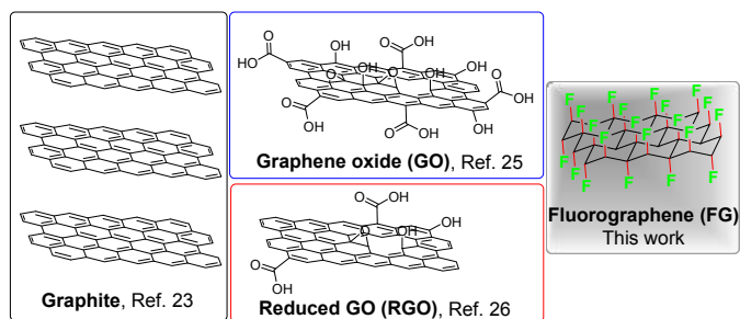
Scheme 1. Structures of the already employed graphene-based carbocatalysts as photochemical promoters for organic transformations.
