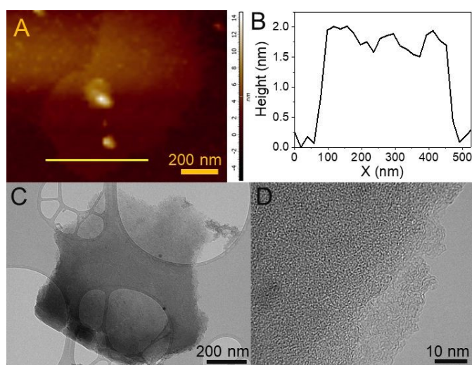
Fig. 1. Panel A shows an AFM image of the dry contents of FG sonicated in MeOH for 30 minutes, with the indicated path of the height profile shown in panel B. Panels C and D show TEM images of the same sample of sonicated FG.
