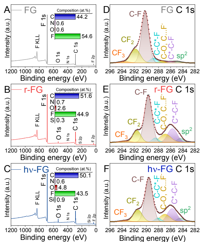
Fig. 4 XPS characterization of exfoliated FG, recovered FG (r-FG), and FG irradiated by LED 456 nm (hv-FG): surveys XPS spectra (A, B, and C, respectively) and C 1s HR-XPS spectra (D, E, and F, respectively).
