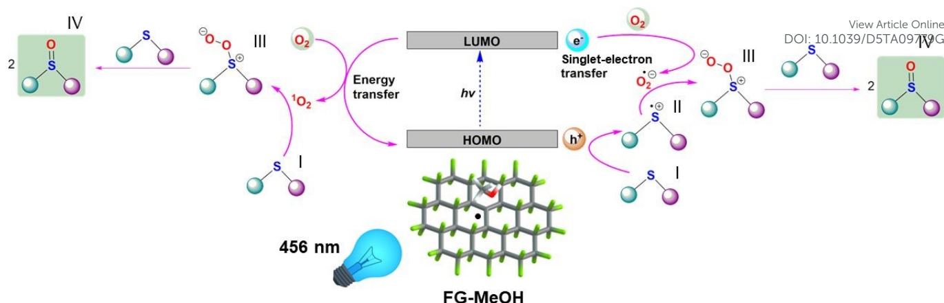
Fig. 3 Proposed mechanisms for the photooxidation of organic sulfides to the corresponding sulfoxides, using FG as a photochemical promoter.
