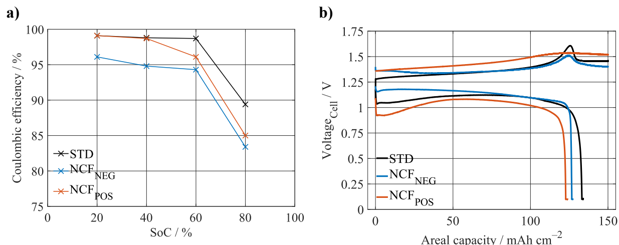
Figure 8: a) CE evolution for the std. construction and the experiment with the NCF NEG and NCF POS half-cell in the ZIHFB. b) ZIHFB voltage dependence on Q_{\text{areal}} for different construction modification (construction modification is captioned in Figure S2 ). Experimental conditions: Std. electrolyte composition: 0.07 dm 3 negolyte, 0.08 dm 3 posolyte; Current density: 100 mA cm -2 ; Operating temperature 40 °C; Electrolyte flow rate: 0.08 dm 3 min -1 .
