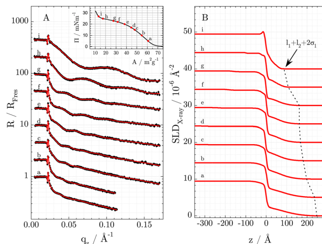
Fig. 5 (A) Fresnel normalised specular X-ray reflectometry of MG particles at the air/water interface and corresponding (B) SLD profiles at the pressures highlighted on the isotherm in the inset in A, starting from the bottom with the lowest lateral pressure. Black symbols are the measured values and red solid lines are the optimised models corresponding to the SLD profiles shown in (B). For improved readability, reflection profiles in (A) are offset by a factor of \sqrt[3]{10} and SLD profiles in (B) are offset by 5 \times 10^{-6} \text{ \AA}^{-2} . The inset displays the sum of the length of the two slabs ( l_1 , l_2 ), including the adjacent transition region ( 2\sigma_1 ) to parameterise the layer present above the apparent air/water interface, as function of \Pi .
