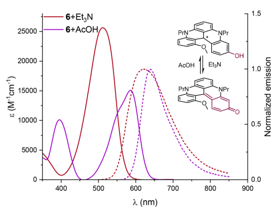
Fig. 7 Absorption and normalized emission spectra of 6 in presence of an excess of either Et 3 N (red) or AcOH (purple) in air-equilibrated MeCN at 20 °C with concentrations of 1 \times 10^{-5} to 3 \times 10^{-5} M.
