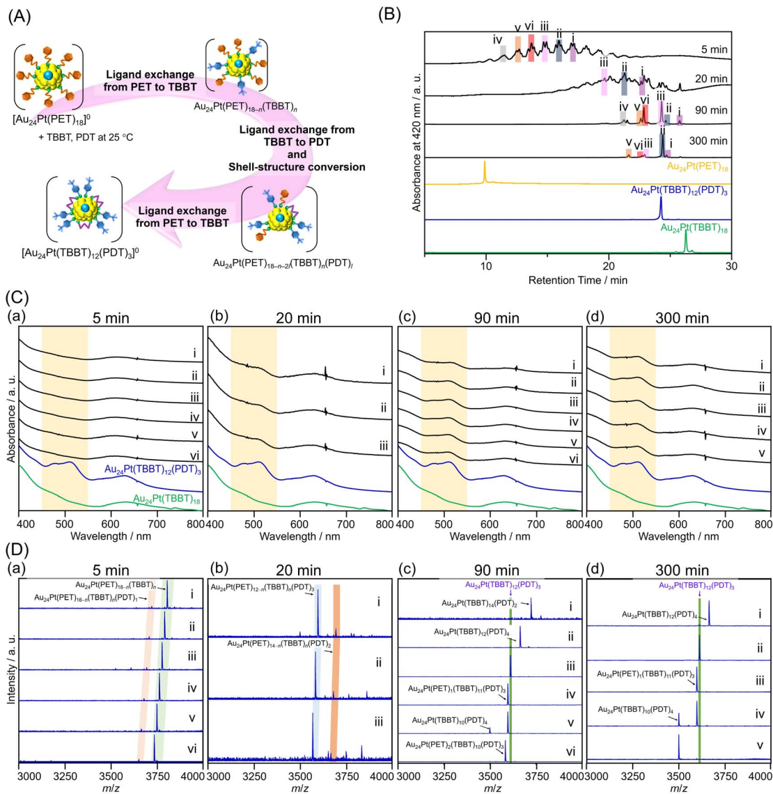
Fig. 4 (A) Schematic illustration of the transformation from [Au 24 Pt(PET) 18 ] 0 to [Au 24 Pt(TBBT) 12 (PDT) 3 ] 0 ; (B) RP-HPLC chromatograms; (C) UV-vis optical absorption spectra obtained with a PDA detector attached to the HPLC apparatus; (D) negative-ion ESI mass spectra of products obtained following the reaction of [Au 24 Pt(PET) 18 ] 0 with TBBT and PDT 2 for (a) 5, (b) 20, (c) 90, and (d) 300 min. Each peak was mainly attributed as follows. At 5 min: (i–vi) Au 24 Pt(PET) 18–n (TBBT) n ( n = 3–8); at 20 min: (i) Au 24 Pt(PET) 1 (TBBT) 11 (PDT) 3 , (ii) Au 24 Pt(PET) 2 (TBBT) 10 (PDT) 3 , (iii) Au 24 Pt(PET) 3 (TBBT) 9 (PDT) 3 ; at 90 min: (i) Au 24 Pt(TBBT) 14 (PDT) 2 , (ii) Au 24 Pt(TBBT) 12 (PDT) 4 , (iii) Au 24 Pt(TBBT) 12 (PDT) 3 , (iv and v) Au 24 Pt(PET) 1 (TBBT) 11 (PDT) 3 , (vi) Au 24 Pt(PET) 2 (TBBT) 10 (PDT) 3 ; at 300 min: (i) Au 24 Pt(TBBT) 12 (PDT) 4 , (ii–iv) Au 24 Pt(PET) 12–n (TBBT) n (PDT) 3 , (v) Au 24 Pt(TBBT) 10 (PDT) 4 .
