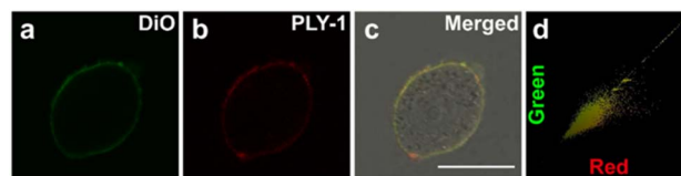
Fig. 4 CLSM images of HeLa cells co-incubated with (a) Dio ( 5.0\text{ }\mu\text{M} , \lambda_{\text{ex}}/\lambda_{\text{em}} = 488\text{ nm}/480 – 530\text{ nm} ), and (b) PLY-1 ( 10.0\text{ }\mu\text{g mL}^{-1} , \lambda_{\text{ex}}/\lambda_{\text{em}} = 405\text{ nm}/600 – 750\text{ nm} ); (c) merged image; (d) intensity correlation plot of Dio and PLY-1. Scale bar: 25\text{ }\mu\text{m} .
