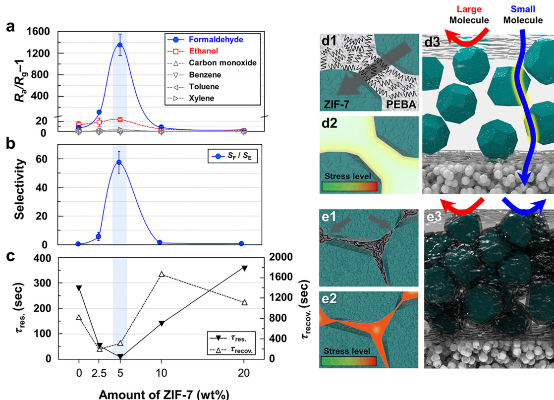
Fig. 35 Gas response, formaldehyde selectivity, response/recovery times, and gas-sensing mechanism. (a) Gas response of pure PEBA/TiO 2 , 2.5MMM/TiO 2 , 5MMM/TiO 2 , 10MMM/TiO 2 , 20MMM/TiO 2 sensors (temperature: 23 °C). (b) Formaldehyde selectivity to ethanol of pure PEBA/TiO 2 , 2.5MMM/TiO 2 , 5MMM/TiO 2 , 10MMM/TiO 2 , 20MMM/TiO 2 sensors. (c) 90% response time ( \tau_{res} , left) and 90% recovery times ( \tau_{recov} , right) of pure PEBA/TiO 2 , 2.5MMM/TiO 2 , 5MMM/TiO 2 , 10MMM/TiO 2 , and 20MMM/TiO 2 sensors. (d) and (e) Schematic illustration of gas penetration model, stress level, and polymer configuration when mild amount of ZIF-7 loading in PEBA (d) and excessively high amount of ZIF-7 loading in PEBA (e). 116 Reproduced with permission from ref. 116, Copyright (2024) American Chemical Society.
