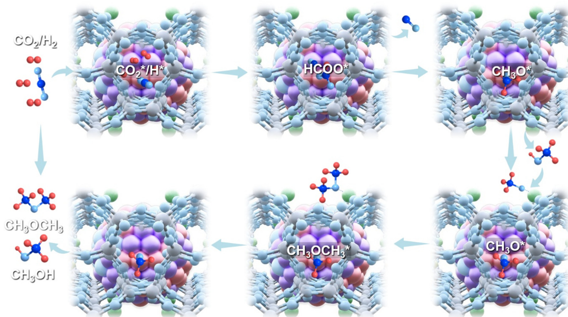
Fig. 5 Proposed reaction mechanisms for \text{CO}_2 hydrogenation to dimethyl ether (DME) and methanol over \text{CZ}(x)\text{@S-t} catalysts.
