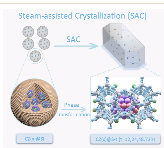
Scheme 1 Schematic synthetic procedures of CZ(x)@S- t catalysts via the SAC method.
