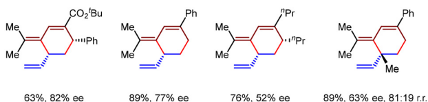
Scheme 21 \text{Pd}(0) -catalyzed asymmetric intermolecular [4+2] cycloadditions of vinylallenes and 1,3-dienes.
