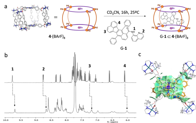
Fig. 1 (a) Schematic representation of the binding of G-1 within cage 4 \cdot (\text{BARF})_8 . (b) Stacked partial ^1\text{H} NMR spectra of G-1 (top) and G-1 \subset 4 \cdot (\text{BARF})_8 (bottom), showing spectral changes upon host-guest complexation. (c) Representation of non-covalent interaction (NCI) surface of encapsulated G-1 within the cage (weak van der Waals interactions in green and stronger interactions in blue).
