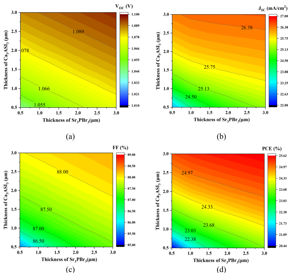
Fig. 3 Role of thickness variation of \text{Sr}_3\text{PBr}_3 and \text{Ca}_3\text{AsI}_3 (device-iii) on the photovoltaic parameters, (a) V_{OC} , (b) J_{SC} , (c) FF, and (d) PCE.
