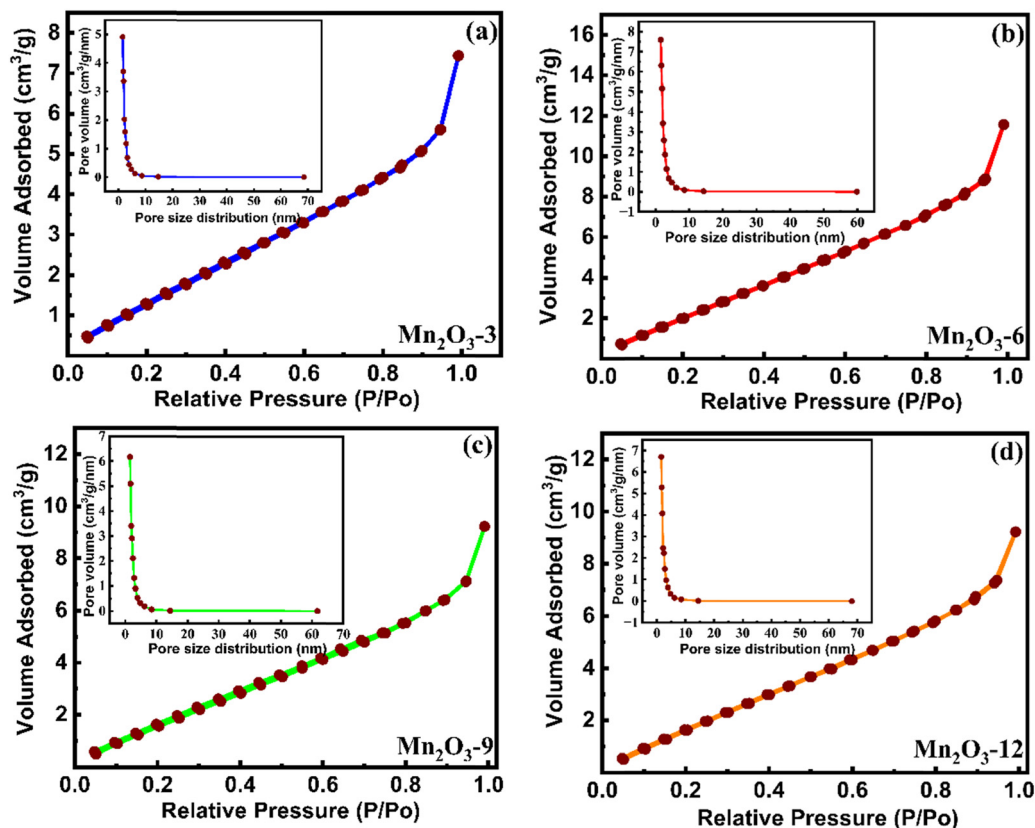
Fig. 4 (a)–(d) \text{N}_2 adsorption and desorption plots of the \text{Mn}_2\text{O}_3 particles measured at 77 K. The inset shows pore size distribution.
