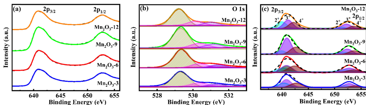
Fig. 5 X-ray photoelectron spectra. (a) High-resolution spectra of Mn 2p, (b) O 1s, and (c) deconvoluted peaks of Mn 2p of \text{Mn}_2\text{O}_3 particles.
