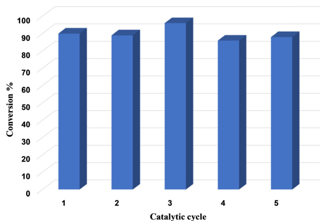
Fig. 2 Reusability of N(Me)_3^+-P5 for multi-cycloaddition cycles using ECH as a substrate; see Fig. S19 (ESI†).
