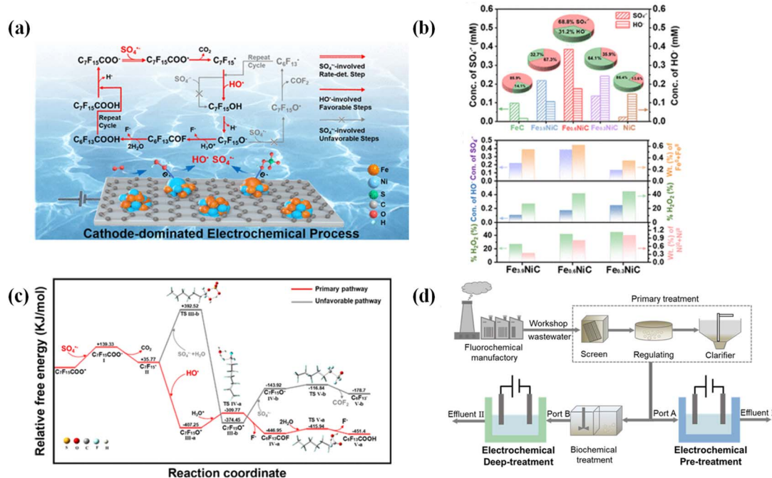
Fig. 16 (a) Schematic of PFOA degradation in a cathode-dominated electro-Fenton process. (b) The quantitative and cumulative concentration of SO_4^{·-} and HO· in different cathodes. (c) Profile of the potential energy surfaces for the PFOA degradation dominated by SO_4^{·-} and HO· . (d) Flowchart of fluorochemical manufactory wastewater treatment. 89
