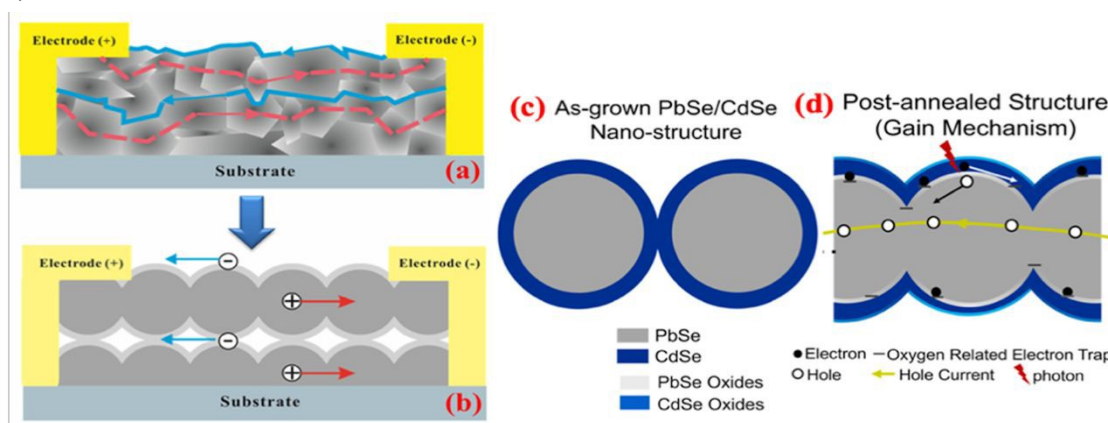
Fig. 4. Conceptual and simulated representations of the charge separation and threading crystallite transport model in sensitized polycrystalline PbSe films. (a) Schematic of p-type to n-type inversion of the surface of crystallites induced by oxygen sensitization, forming a core-shell structure. (b) Idealized polycrystalline geometry used in the numerical model, where each sphere represents an individual crystallite and its corresponding grain boundary environment. (a) and (b) are adapted from B. Weng et al., Proc. SPIE, 2013, 8993, 8993–37, with permission from SPIE. 84 (c) Pristine core-shell morphology showing spatial separation of electrons and holes across the PbSe/CdSe interface. (d) Optimized structure exhibiting vertically aligned (threaded) PbSe cores, enabling long-range hole transport, injection of new carriers, and recombination suppression by confining minority electrons to the shell. (c) and (d) are adapted from R. M. Mirzaei and Z. Shi, Appl. Phys. Lett., 2024, 125 (8), with the permission of AIP Publishing. 83
