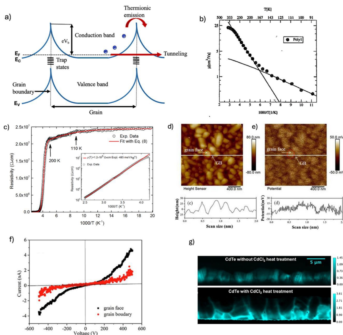
Fig. 3. a) Schematic energy band diagram illustrating that thermionic emission occurs as carriers overcome grain boundary (GB) potential barriers formed by trap states ( N_t ), with possible tunneling contribution under strong fields. b) Arrhenius plot of Hall mobility in polycrystalline CuGaSe 2 thin films, showing three temperature-dependent transport regimes: (I) high-temperature bulk-limited conduction, (II) intermediate-temperature thermionic emission over GB barriers (150K–300K), and (III) low-temperature hopping between localized states. Adapted b) with permission from S. Schuler, "Charge carrier transport in polycrystalline CuGaSe 2 thin films," IEEE Proceedings, 2002. © 2002 IEEE. 25 c) Temperature-dependent resistivity in Sb 2 Se 3 fitted with a thermionic emission model in region II (200K–110K), yielding a GB barrier height of \sim 391 meV and a trap density of 3.4 \times 10^{11} \text{ cm}^{-2} ; flattening at low temperature ( T < 110\text{K} ) indicates transition to hopping-assisted transport (region III). Adapted with permission from N. Cifuentes et al., J. Phys. Chem. C, 2020, 124 (14), 7677–7682. Copyright 2020 American Chemical Society. 52 d) AFM topography and (e) KPFM surface potential image of NiO film highlighting nanoscale potential dips at grain boundaries, indicating the presence of electrostatic barriers, f) Local I–V curves measured by C-AFM across grain face and grain boundary regions in NiO show suppressed current at GBs, consistent with thermionic-limited transport under moderate bias. (d), (e) and (f) are adapted from Yidong Zhang et al., Physica E: Low-dimensional Systems and Nanostructures, 2019, 111, 75–78, with permission from Elsevier. 54 g) EBIC images of CdTe before and after CdCl 2 treatment reveal enhanced carrier collection along GBs post-passivation, attributed to barrier height reduction and improved thermionic emission across GBs. Adapted with permission from Chen Li et al., Phys. Rev. Lett., 2014, 112, 156103. © 2014 American Physical Society. 57
