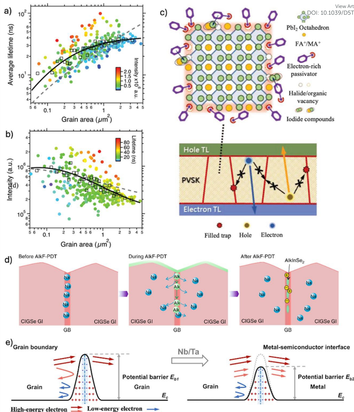
Fig. 6. The influence of grain size, trap states, and passivation strategies on carrier transport in polycrystalline semiconductors. (a–b) Fluorescence lifetime imaging microscopy (FLIM) analysis of ~300 perovskite grains reveal that smaller grains exhibit shorter photoluminescence (PL) lifetimes and reduced intensity, indicating increased trap-assisted non-radiative recombination at GBs. a) and b) are adapted from Mengjin Yang et al., Phys. Chem. Chem. Phys. , 2017, 19, 5043–5050, with permission from the Royal Society of Chemistry. 93 c) Schematic illustration of how electron-rich molecular passivators mitigate defect states (e.g., halide vacancies) and suppress trap-assisted recombination by stabilizing interfacial electron clouds at the perovskite grain surfaces. Adapted from Qihuang Gong et al., Adv. Mater. , 2020, 32 (39), 2005506. Licensed under CC BY 4.0 ( https://creativecommons.org/licenses/by/4.0/ ). 46 d) Post-deposition treatment (PDT) in CIGSe films enables passivating recombination-active sites and enhancing charge collection. Adapted from Nicoleta Nicoara, X. Fu, T. P. Weiss, et al., Nat. Commun. , 2019, 10, 3980. Licensed under CC BY 4.0 ( https://creativecommons.org/licenses/by/4.0/ ). 97 e) Schematic illustration showing the difference in interfacial potential barriers ( E_b ) at a conventional grain boundary and at a metal–semiconductor interface in n-type \text{Mg}_3(\text{Sb,Bi})_2 . The metal inclusion reduces the barrier height and promotes carrier transmission across the interface. Adapted from Li et al., Nature Communications , 2023, 14, 7428. Licensed under CC BY 4.0 ( https://creativecommons.org/licenses/by/4.0/ ). 15
