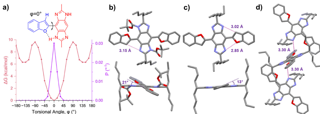
Fig. 3 (a) Relative energy ( \Delta G ) and probability density ( P ) obtained through torsional analysis by rotating 15^\circ across the bridging \text{C-C} bond of a benzobisimidazole–benzofuran system using density functional theory at B3LYP/6-31G(d) level of theory; (b)–(d) front view (top) and side view (bottom) of single molecule crystal structures of 4 and 5 , as well as crystal packing of 5 showing intermolecular hydrogen-bonding interactions.
