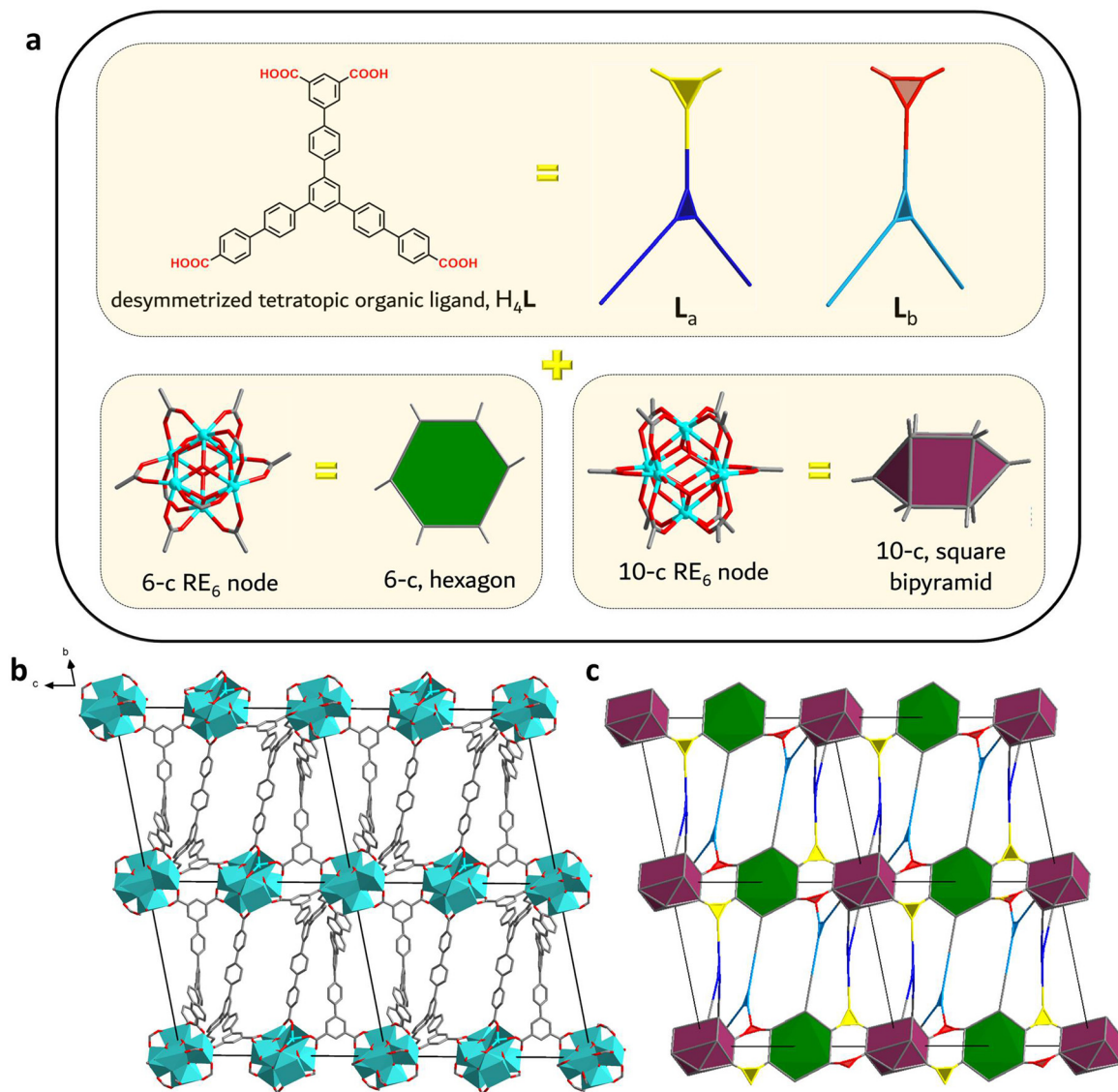
Fig. 2 (a) The combination of the desymmetrized, tetratopic H_4L organic linker with 6-c and 10-c RE_6 -clusters resulted in the formation of RE - stc -MOF-1 series of MOFs. Their geometric representation used for the topological analysis is shown where crystallographically distinct components have different colors. (b) The structure of Eu - stc -MOF-1 looking down the a -axis. (c) The unique six nodal, (3,3,3,3,6,10)-c, augmented stc -a net derived from the topological analysis of Eu - stc -MOF-1.
