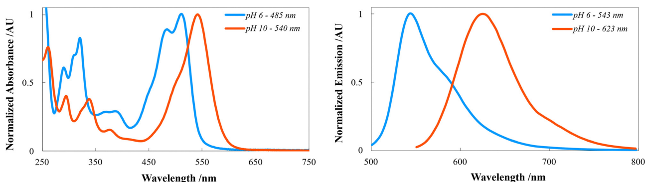
Fig. 1 Normalized absorption and emission spectra of SNAFL-C at pH 6 (naphthol, PBS buffer, \lambda_{\text{ex}} = 485 nm) and pH 10 (naphtholate, carbonate/bicarbonate buffer, \lambda_{\text{ex}} = 540 nm).
