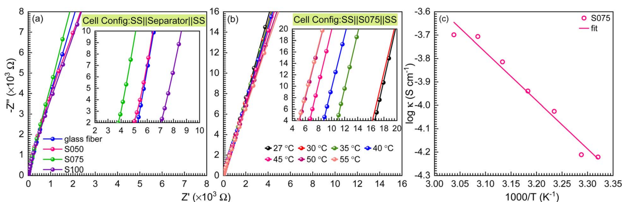
Fig. 4 (a) The Nyquist plot for all the separators at room temperature; (b) the Nyquist plot for the control, S075 membrane at the various temperatures (27 ^{\circ}\text{C} , 30 ^{\circ}\text{C} , 35 ^{\circ}\text{C} , 40 ^{\circ}\text{C} , 45 ^{\circ}\text{C} , 50 ^{\circ}\text{C} , 55 ^{\circ}\text{C} ), using a blocking electrode system (SS||separator||SS); (c) the ionic conductivity values for the S075 separator at the different temperatures.
