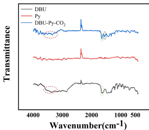
Fig. 5 FT-IR spectra of DBU, Py, and DBU-Py-CO 2 .
