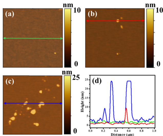
Fig. 7 Atomic force microscopy (AFM) images of (a) pure Lys PG monolayer, and Lys PG monolayer in the presence of (b) 20 mol% UBI (29–41), and (c) 20 mol% UBI-2-APBA. (d) Corresponding height profiles of all three systems following the lines shown in the AFM images. The profiles represent the height from the lipid monolayer surface, not from the underlying Si-substrate. Monolayers were transferred onto silicon substrates using the Langmuir–Blodgett technique at a surface pressure of 30 mN \text{m}^{-1} . The AFM topography images have a scan size of 1 \times 1 \mu\text{m}^2 .
