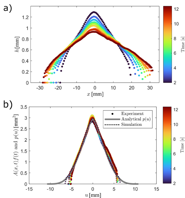
Fig. 3 (a) Droplet profiles for an experiment with XG concentration of 2 \text{ g L}^{-1} for 9 different times in the range t = 2.0\text{--}12.4 \text{ s} shown in the colorbar. (b) The dots show the experimental values of A(x, t) f(t) . The analytical result for the function p(u) of eqn (17) using the value n = 0.48 is plotted as a gray line, while the simulations that take the finite corner curvature h_0 = 0.6 \text{ mm} and initial profile half-width w_0 = 0.8 \text{ mm} , are shown for the initial and final times. The diffusion constant resulting from the data fit is D_0 = 200 \text{ mm}^{1/n} \text{ s}^{-1} .
