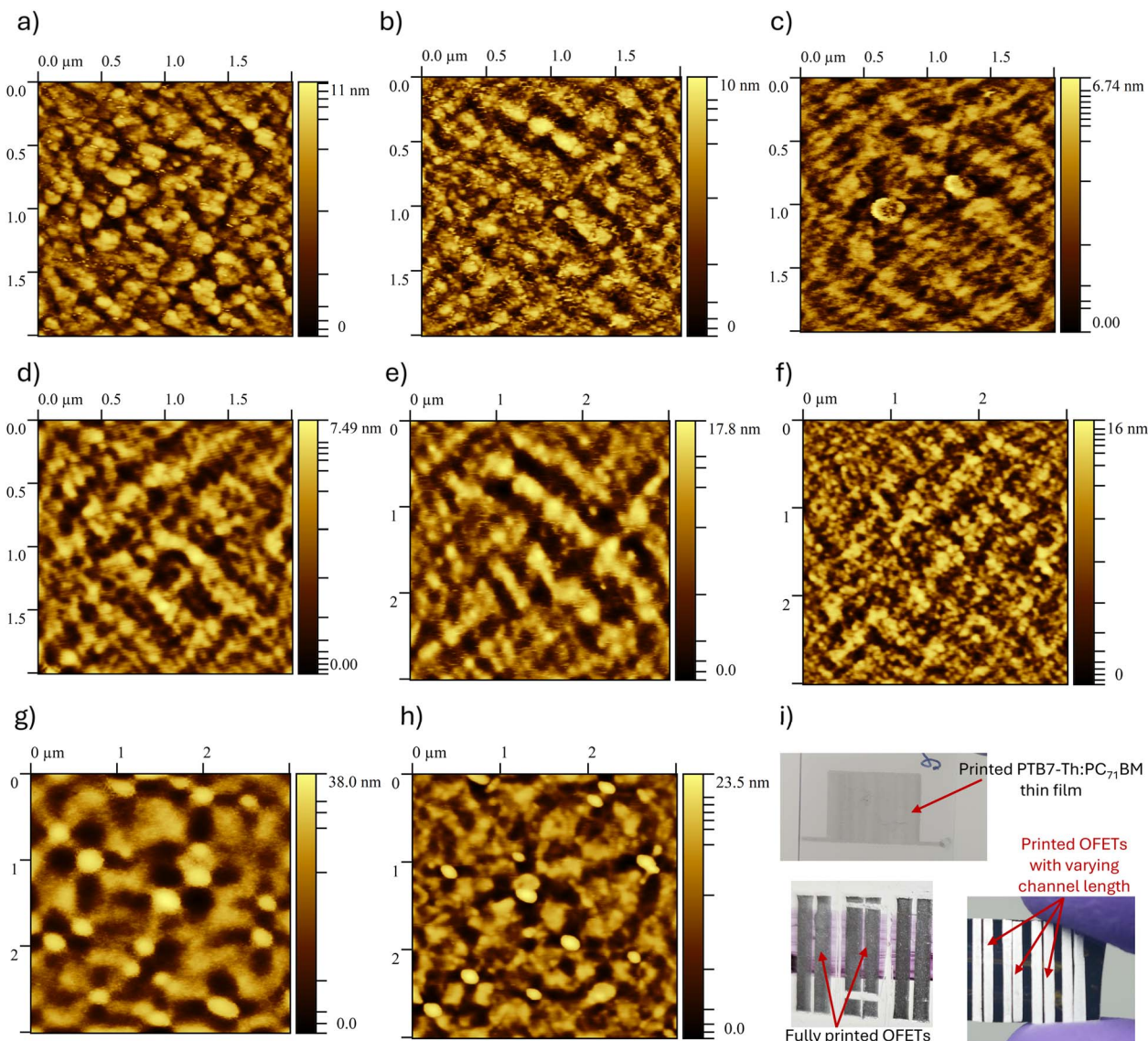
Fig. 3 AFM topographic images ( 2\ \mu\text{m} \times 2\ \mu\text{m} ) – (a) and (b) ZnO printed, and spin-coated respectively, and (c) and (d) PTB7-Th:PC 71 BM blend printed, and spin coated, respectively; ( 3\ \mu\text{m} \times 3\ \mu\text{m} ) – (e) and (f) PBTTT-C14 on gelatin/ITO printed and spin coated, respectively; (g) and (h) PBTTT-C14 on OTS-treated Si/SiO 2 printed and spin coated, respectively and (i) snapshots (top–bottom clockwise) of printed PTB7-Th:PC 71 BM thin films on a glass substrate, OFETs with printed PBTTT-C14 and top S-D electrodes using Ag ink with OTS-treated SiO 2 as the gate dielectric, and OFETs with all the layers printed, including gelatin gate dielectric, PBTTT-C14 active layer, and top S-D Ag electrodes.
