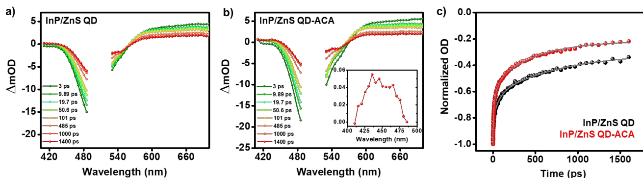
Fig. 2 fs-TA spectra at indicated time delays upon 500 nm excitation of a) InP/ZnS QDs and b) InP/ZnS QD-ACA. Inset of (b) shows the absorption feature of ^3\text{ACA}^* at ~430 nm obtained by subtracting the normalized spectra corresponding to 1400 ps and 3 ps time delays. c) Kinetics of the GSB bleach recovery of InP/ZnS QDs with and without ACA ligands.
