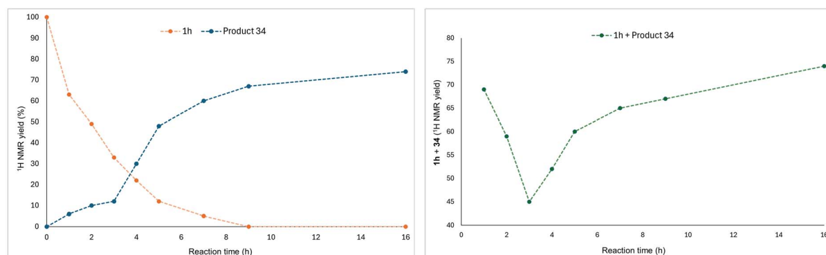
Fig. 4 (A) Radical trapping and inhibition experiment. (B) Kinetic isotope effect (KIE). (C) Proposed mechanism. (D) Left: Temporal evolution of 4-chlorostyrene (1h, orange) and oxo-amidomethylated product 34 (blue); Right: Temporal evolution of combined starting material (1h) and product 34 (mass balance).
