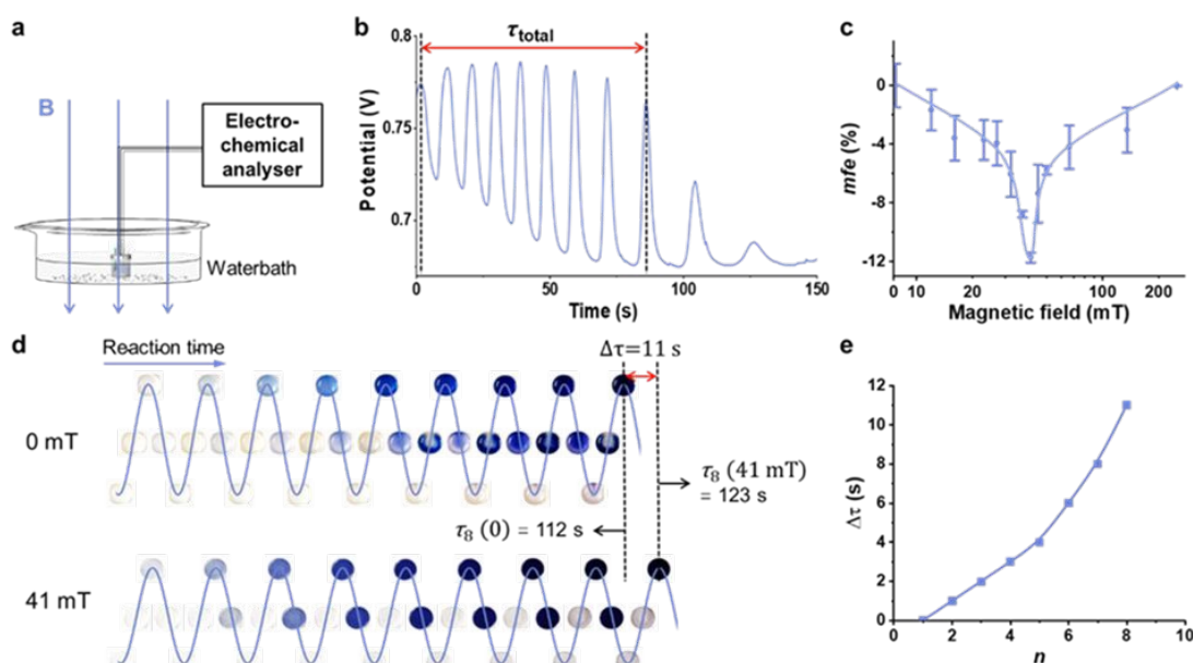
Fig. 1 Experimental setting and MFEs on BR oscillation. a, The sample cell ( 1 \times 1 \times 1 \text{ cm} ) was placed 0.5 m from the centre of the magnet. b, Potential versus time plot. c, Relative k_{\text{obs}} of the BR reaction as a function of applied MF, the error bars represent the standard deviations of 3 independent measurements. d, Images of the BR oscillation at 0 mT and 41 mT recorded by video. e, The period difference between 41 mT and 0 mT varies with the oscillation number ( n ).
