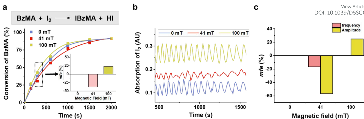
Fig. 2 MFs on the conversion of BzMA. a, Time trace of the BzMA conversion measured by HPLC at 0 mT (blue line), 41 mT (red line), and 100 mT (green line). b, Time trace of I_2 absorbance (460 nm) in BzMA oscillating systems at 0, 41, and 100 mT. c, Comparison of mfe between frequency and amplitude in Fig. 2b.
