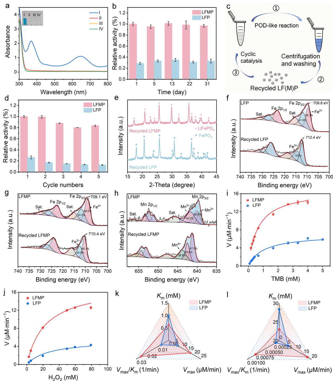
Fig. 3 (a) UV absorption spectra and corresponding photographs (inset) of TMB under different conditions. LFMP + H_2O_2 + TMB (I); LFMP + TMB (II); H_2O_2 + TMB (III); TMB (IV). (b) Relative activity of LFMP and LFP versus storage time. (c) The flowchart of the cyclic catalysis process of LF(M)P. (d) Relative activity of LFMP and LFP for TMB oxidation after several catalytic cycles. (e) XRD patterns of cycled LFP and LFMP. Reaction conditions for panels a to d: H_2O_2 (10 mM), TMB (0.42 mM), LFMP or LFP (50 \mu\text{g mL}^{-1} ), 0.2 M phosphate solution (pH = 4), 5 min reaction. Fe 2p spectra of LFP (f) and LFMP (g) before reaction and after five cycles of catalysis. (h) Mn 2p spectra of LFMP and recycled LFMP. Michaelis–Menten curves of LFMP and LFP with TMB (i) and H_2O_2 (j) as substrates, respectively. Radar plots of the three parameters ( K_m , V_{max} , and V_{max}/K_m ) of LFMP and LFP with TMB (k) and H_2O_2 (l) as substrates, respectively. Reaction conditions for panels i to l: LFMP or LFP (10 \mu\text{g mL}^{-1} ), 0.2 M phosphate solution (pH = 4), 5 min reaction. For panels i and k: H_2O_2 (50 mM). For panels j and l: TMB (1.68 mM).
