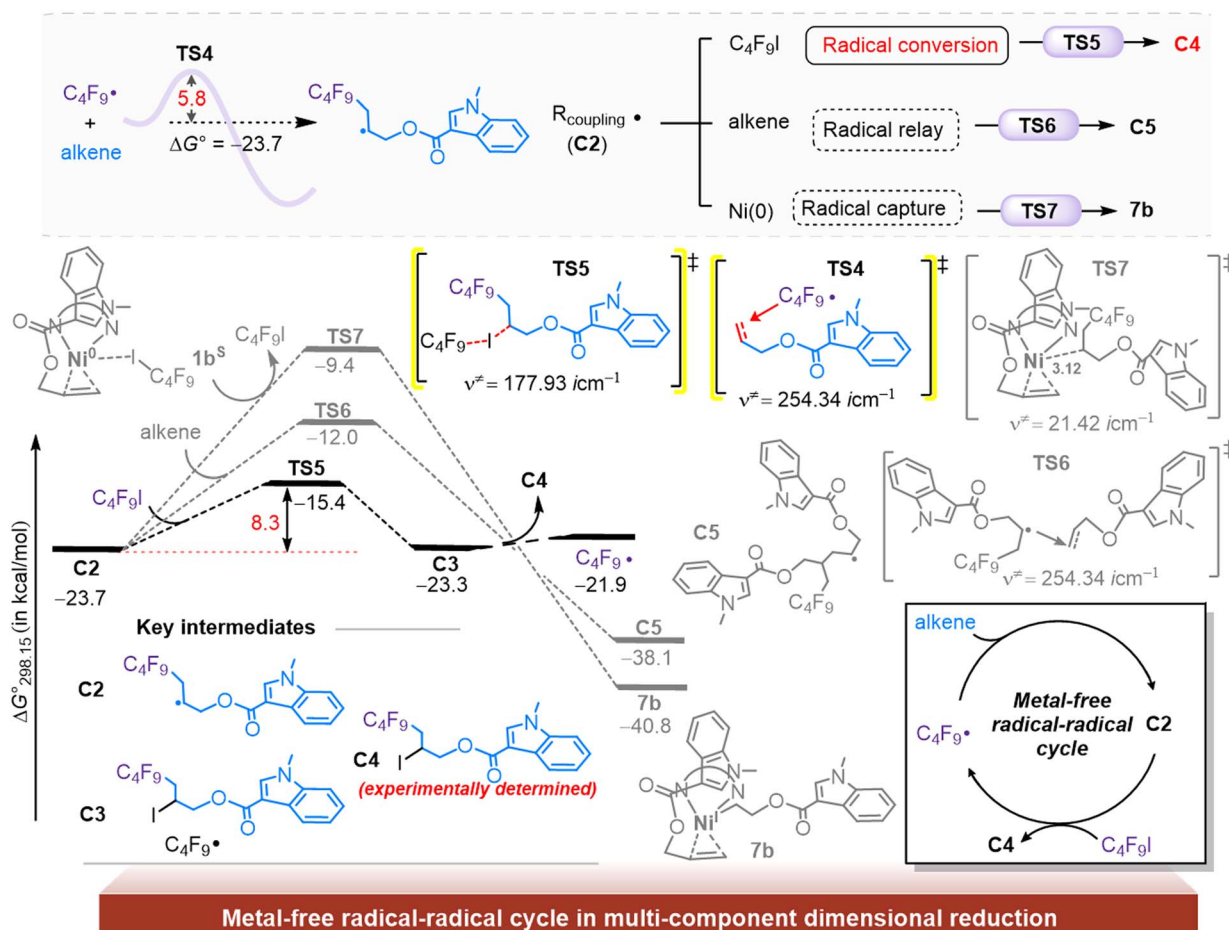
Fig. 3 Gibbs energy profile (in \text{kcal mol}^{-1} ) of polymerization and termination of radicals to form a two-component coupled intermediate C4. Red numbers indicate Gibbs activation energies for the corresponding steps, and the fluorescent yellow line marks the most favorable pathway.
