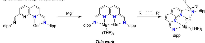
Scheme 1 (a–c) The various types of reactivity modes described for germylenes and (d) the Ge-main group cooperativity described in this work.
