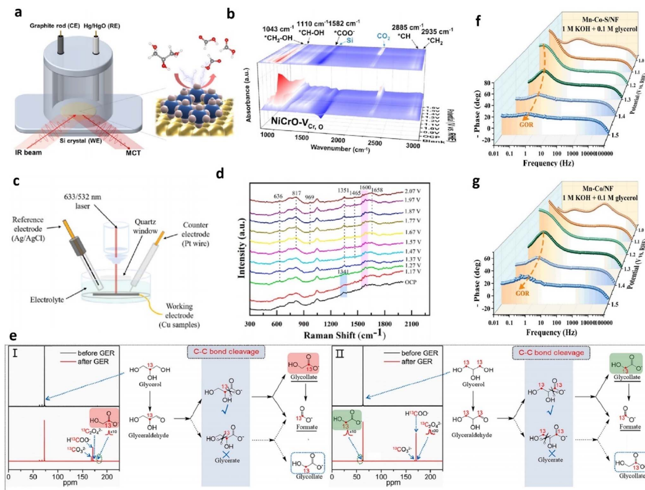
Fig. 5 (a) Illustration of in situ ATR-SEIRAS. (b) In situ ATR-SEIRAS spectra of the GOR on NiCrO-V- \text{Cr}_2\text{O}_3 nanosheet electrodes at various potentials. Reproduced from ref. 63, copyright 2024, American Chemical Society. (c) Schematic diagram for in situ Raman measurements. (d) In situ electrochemical Raman spectra on Cu NPs in 0.1 M KOH with 0.1 M glycerol solution. Reproduced from ref. 70, copyright 2023, Elsevier. (e) ^{13}\text{C} -NMR spectra for the electrooxidation of isotope-labelling (I) 2\text{-}^{13}\text{C} glycerol and (II) 1,3\text{-}^{13}\text{C} glycerol. Reproduced from ref. 60, copyright 2023, Elsevier. Bode plots of Mn-Co-S/NF (f) and Mn-Co/NF (g) for the GOR. Reproduced with permission from ref. 66, copyright 2024, Elsevier.
