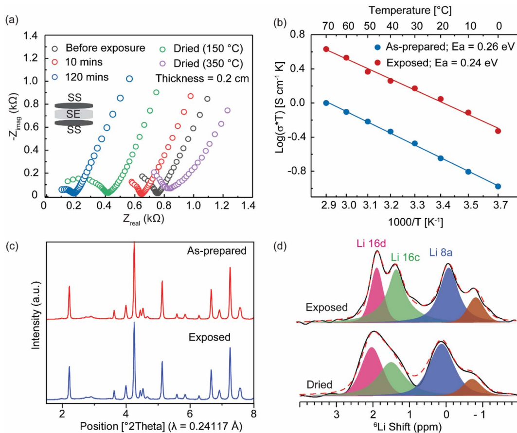
Fig. 5 (a) Nyquist plot for the as-prepared, humid-air-exposed, and dried \text{Li}_{3.6}\text{In}_7\text{S}_{11.8}\text{Cl} . (b) Arrhenius plot and the extracted activation energy ( E_a ) for ion transport in as-prepared and humid-air-exposed \text{Li}_{3.6}\text{In}_7\text{S}_{11.8}\text{Cl} . (c) XRD patterns for as-prepared and air/moisture-exposed \text{Li}_{3.6}\text{In}_7\text{S}_{11.8}\text{Cl} . (d) ^6\text{Li} MAS NMR spectra of humid-air-exposed and dried \text{Li}_{3.6}\text{In}_7\text{S}_{11.8}\text{Cl} .
