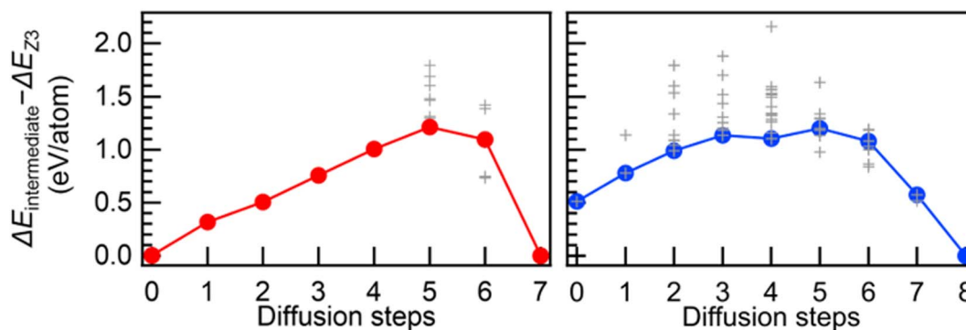
Fig. 7 Formation energies of intermediate structures ( \Delta E_{\text{intermediate}} ) compared with Z3 - \text{Fe}_8\text{Pd}_{20}\text{In}_4 ( \Delta E_{Z3} ), where the red and blue curves are the diffusion paths with the minimum formation energies formed from L1_2 - \text{Fe}_4\text{Pd}_{24}\text{In}_4 and L1_0 - \text{Fe}_{16}\text{Pd}_{16}/bct - \text{Pd}_{24}\text{In}_8 , respectively, and the + marks represent other paths.
