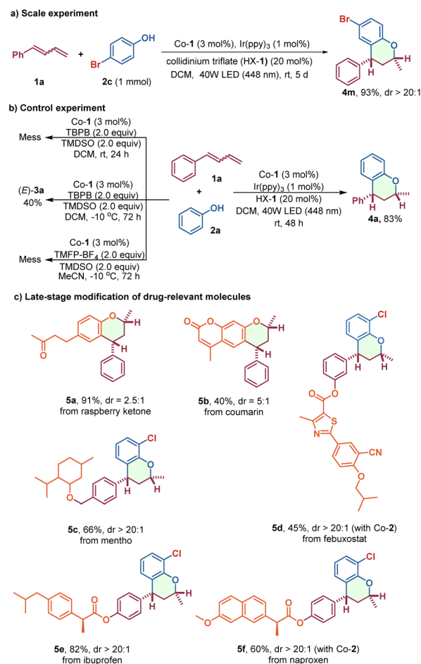
Scheme 4 Synthetic applications.
