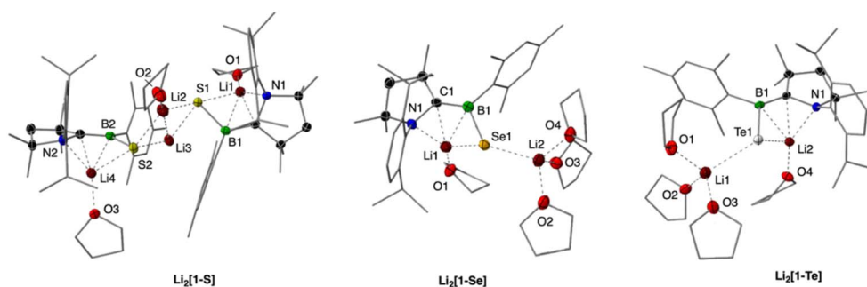
Fig. 4 Molecular structures of the dianions Li_2[1-S] , Li_2[1-Se] , and Li_2[1-Te] . Thermal ellipsoids set at 50% probability. For clarity, hydrogen atoms are omitted, along with the thermal ellipsoids for the substituents and thf molecules. For a comparison of key bond parameters, refer to Table S2 in the ESI.†
