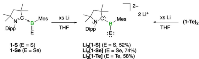
Scheme 4 Synthesis of the dilithium salts Li_2[1-E] (E = S, Se, and Te) by two-electron reduction of the neutral boron chalcogenides. The Lewis structures of the dianions illustrate their valence electrons.
