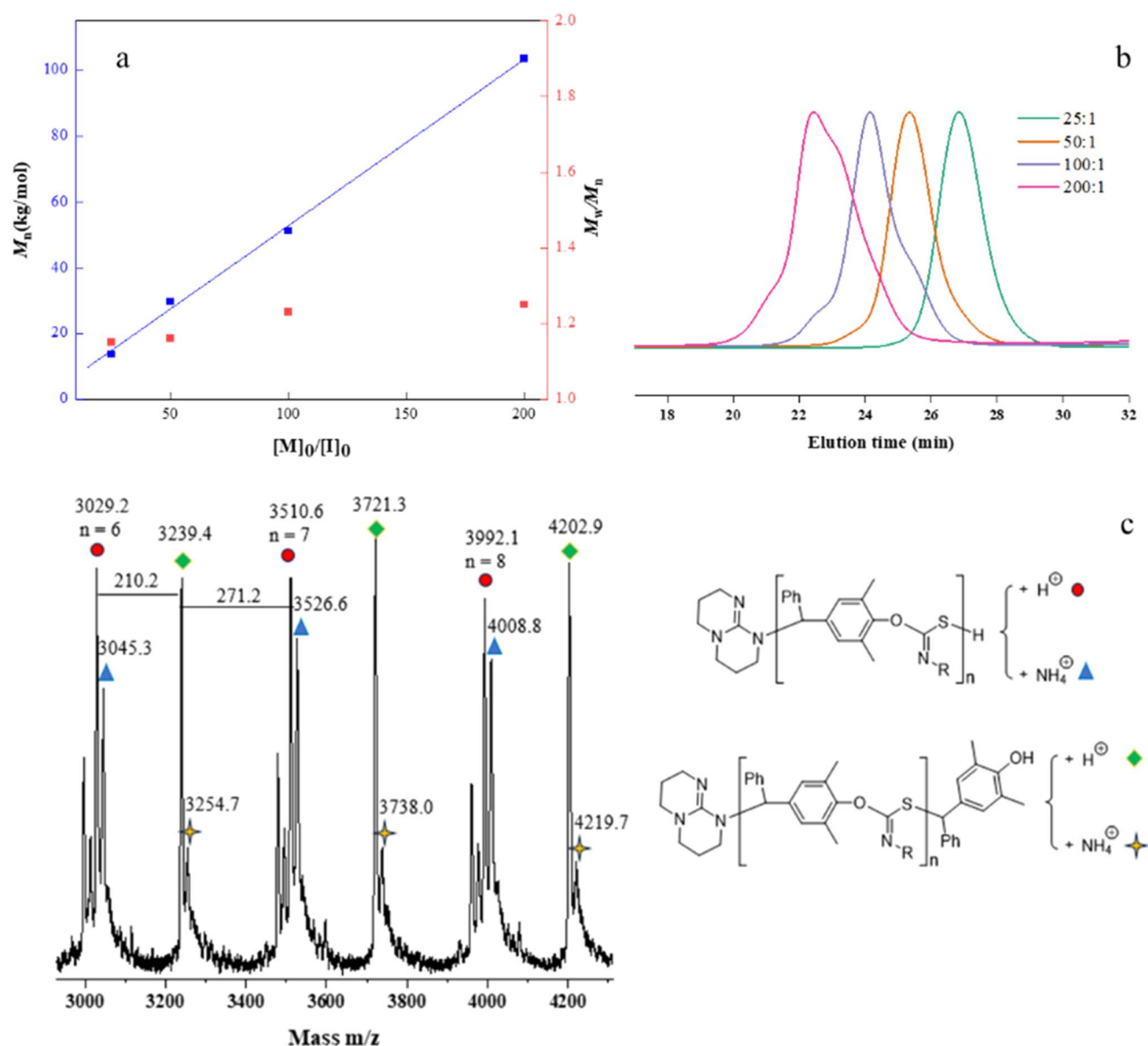
Fig. 1 (a) Plots of M_n and \bar{D} vs. the [p\text{-QM}]_0/[\text{TBD}]_0 ratio; (b) SEC traces of copolymers (color online); (c) MALDI-TOF MS spectrum of the low-molecular-weight p -QM-alt- 1a .
