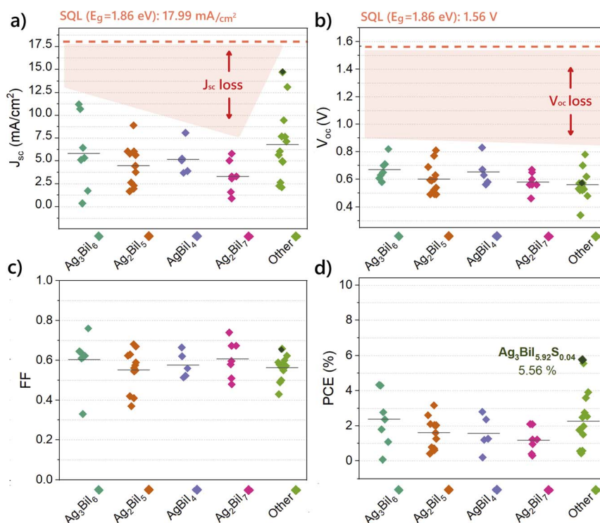
Fig. 3 Electrical parameters J_{sc} (a), V_{oc} (b), FF (c), and PCE (d) for the most common SBI compounds Ag_3BiI_6 , Ag_2BiI_5 , AgBiI_4 , Ag_2BiI_7 , and other SBI-related compounds reported over the years (full table is given in ESI, Table S1†). For reference, dashed lines refer to the values of the SQL theoretical limit for Ag_2BiI_5 ( E_g : 1.86 eV 49 ). Parameters of the champion SBI solar cell are marked in dark green.
