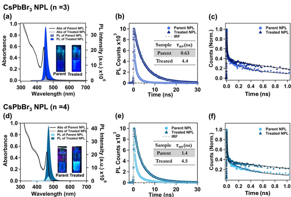
Fig. 2 Optical properties of CsPbBr 3 NPLs ( n = 3 ) before and after OAmF treatment. (a) The UV-visible absorption and PL spectra. (b) PL decay. (c) Femtosecond time-resolved PL decay. (d) The UV-visible absorption and PL spectra, (e) PL decay and (f) femtosecond time-resolved PL decay of parent and treated CsPbBr 3 NPLs ( n = 4 ). All PL spectra were recorded upon exciting the sample at 350 nm. The nanosecond and femtoseconds PL transients were recorded by exciting the sample at 375 nm and 400 nm, respectively.
