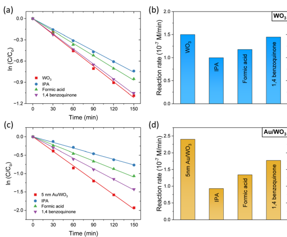
Fig. 8 IBU photodegradation kinetics and reaction rates for (a) and (b) pristine \text{WO}_3 and (c) and (d) 5 nm Au/WO 3 IO photocatalysts in the presence of IPA, formic acid, and 1,4-benzoquinone radical scavengers in 0.1 M NaHCO 3 supporting electrolyte at +1.5 V vs. Ag/AgCl under UV-Vis irradiation.
