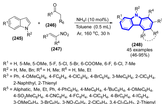
Scheme 68 Synthesis of carbazoles catalyzed by NH 4 I.
