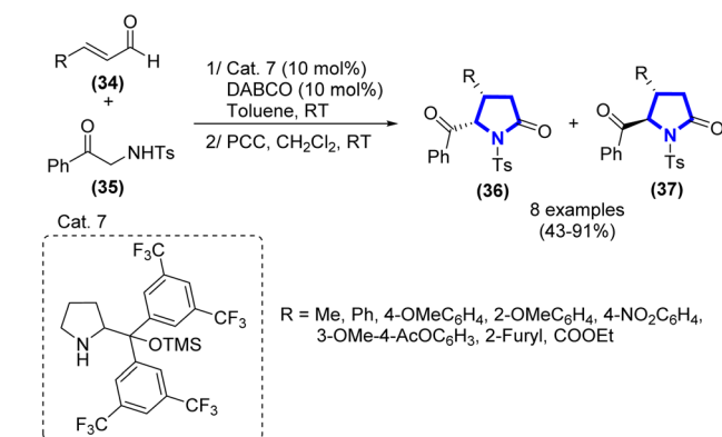
Scheme 10 Synthesis of \alpha -amino- \delta -keto esters or \beta -substituted \delta -oxoamides catalyzed by Cat. 7 .
