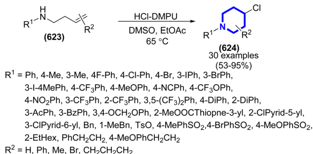
Scheme 170 Synthesis of piperidines catalyzed by HCl/DMU.
