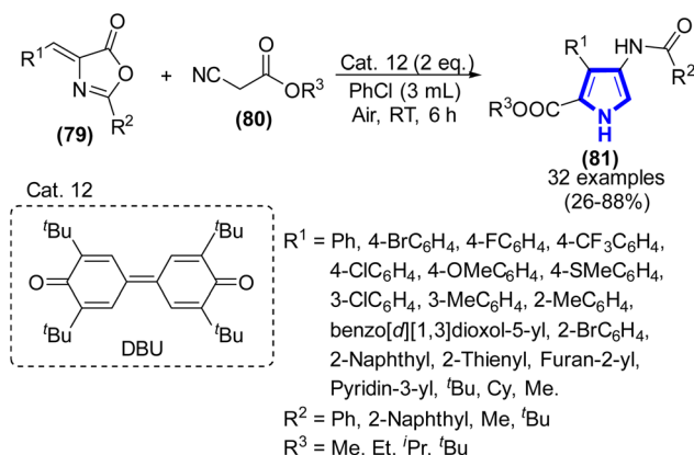
Scheme 21 Preparation of 2,3,4-trisubstituted pyrroles catalyzed by Cat. 12.
