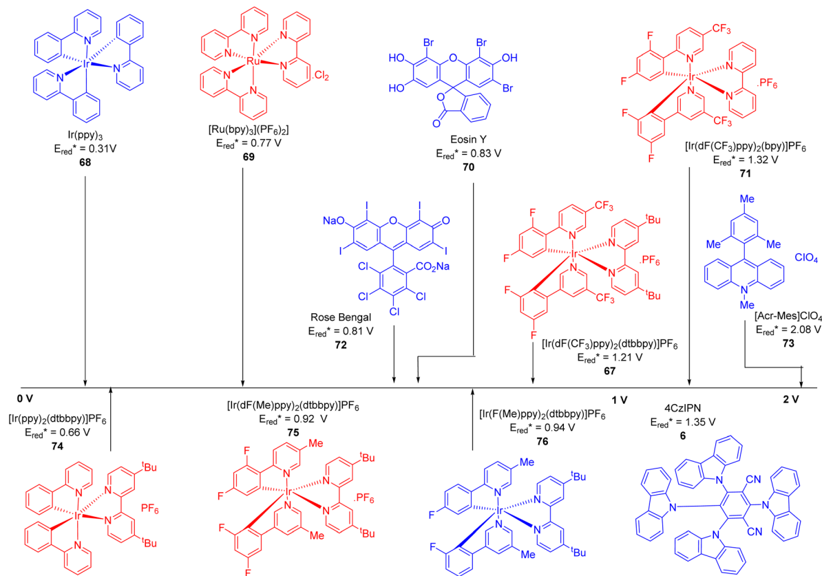
Fig. 48 E_{red}^* of common visible light PCs. Reproduced from ref. 208, https://doi.org/10.1039/D1CS00198A , under the terms of the CC BY-NC 3.0 license, https://creativecommons.org/licenses/by-nc/3.0/ .
