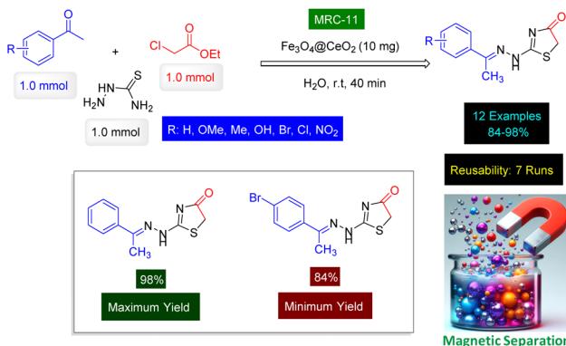
Scheme 11 \text{Fe}_3\text{O}_4 @CeO 2 nanomaterial (MRC-11) catalyzed preparation of thiazole derivatives from thiosemicarbazide.
